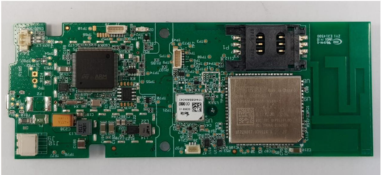
Fig. 8 PC Board Front View with Controller Circuitry Cover Removed
