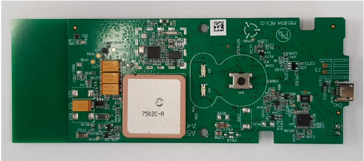
Fig. 10 PC Board Back View with BLE Circuitry Cover Removed
