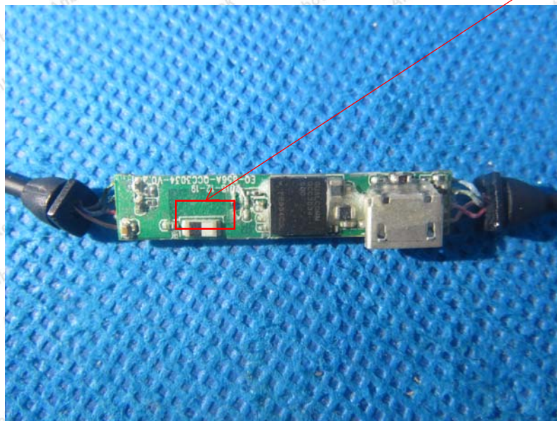
BT Antenna
