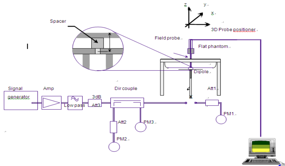
Fig 7.1 System Setup for System Evaluation
