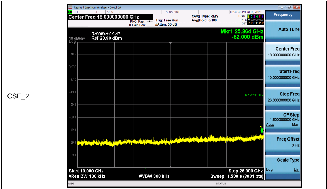
RF Conducted Spurious Emissions_DH5_2441
