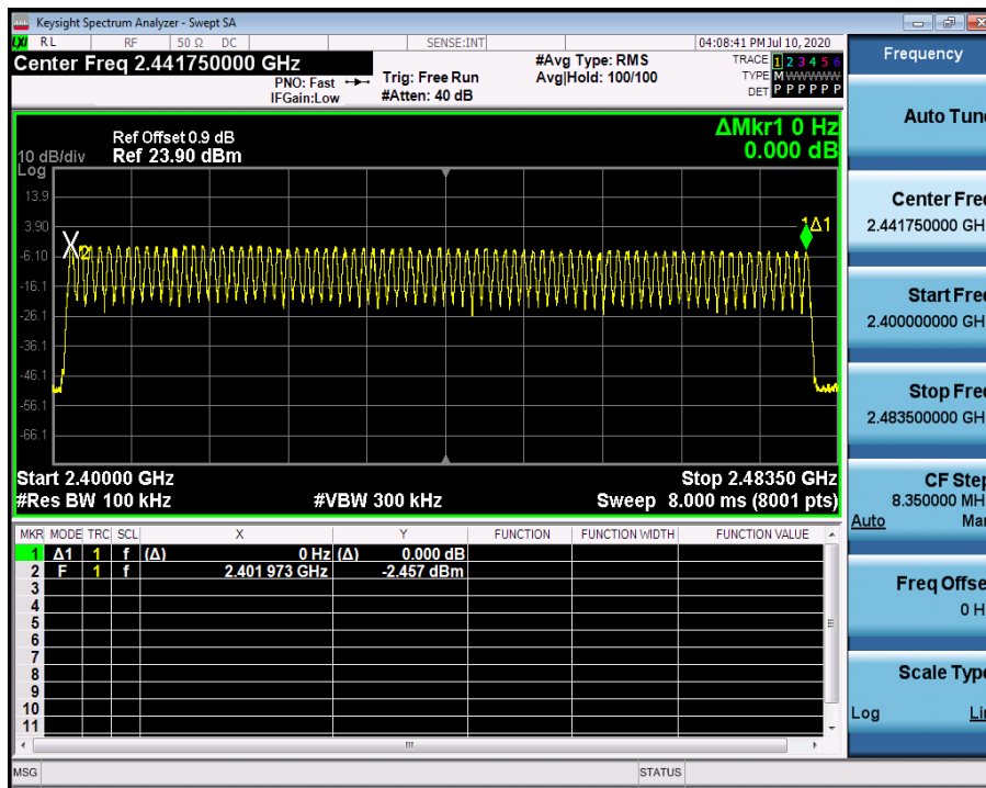
Hopping Channel Number_DH5_2402
