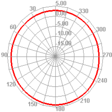
Bluetooth 39 TRP H
