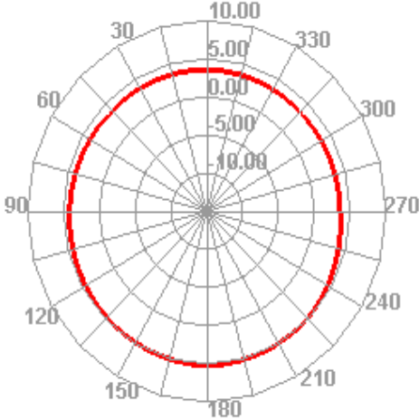
Bluetooth 78 TRP H
