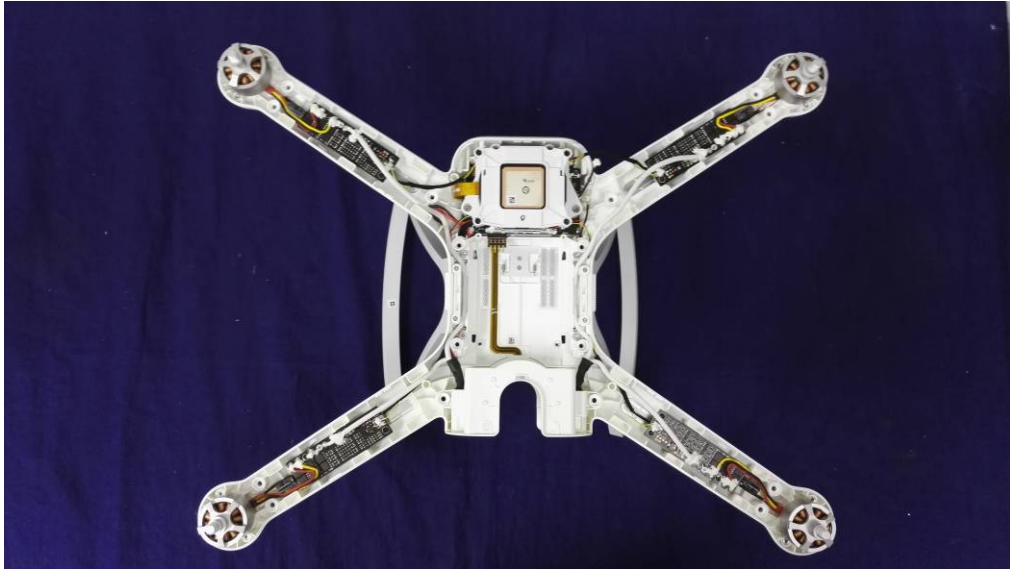
(1) EUT Photo
