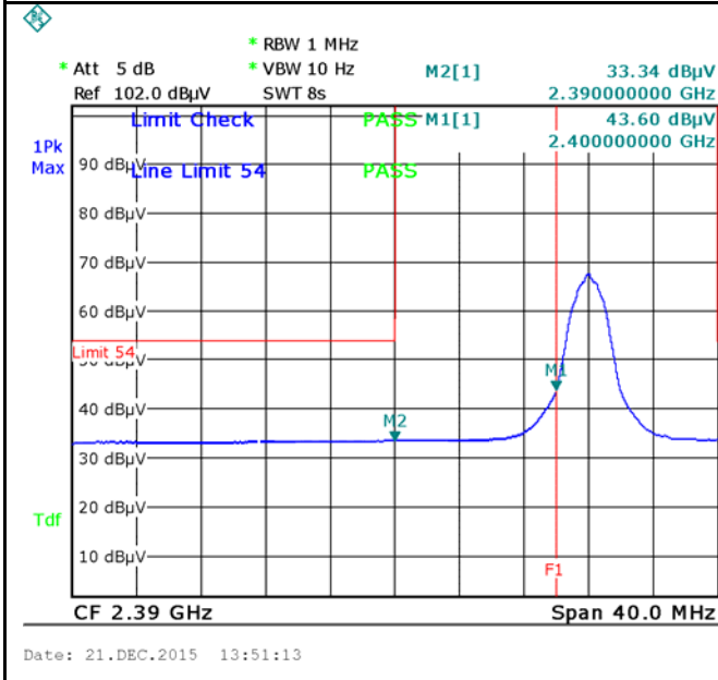
\pi / 4 DQPSK-Left Side-AV Note: F1 is frequency 2400MHz
