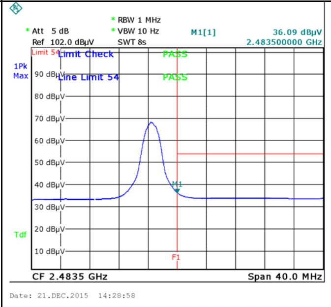
\pi / 4 DQPSK-Right Side-AV Note: F1 is frequency 2483.5MHz
