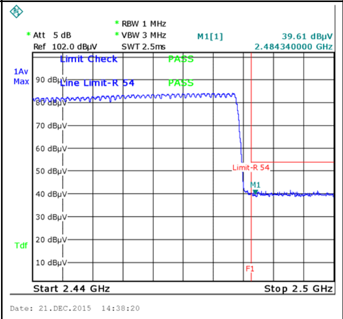
GFSK-Hopping Right Side-AV Note: F1 is frequency 2483.5MHz
