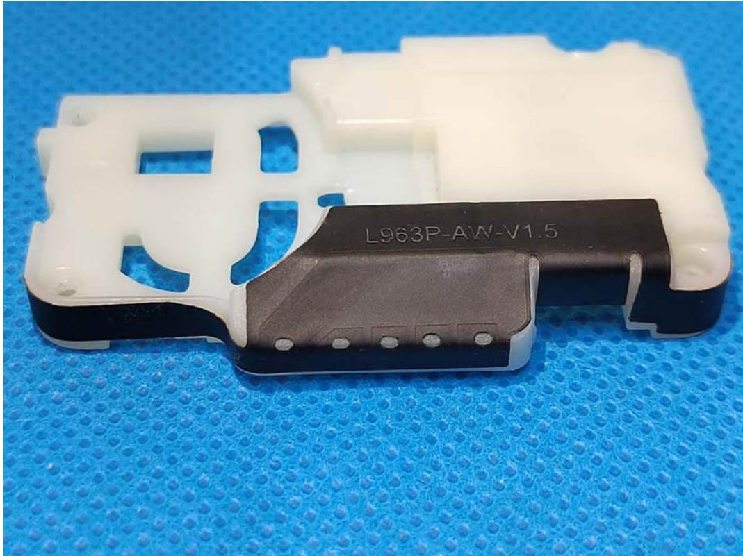
2G/3G/4G Antenna
