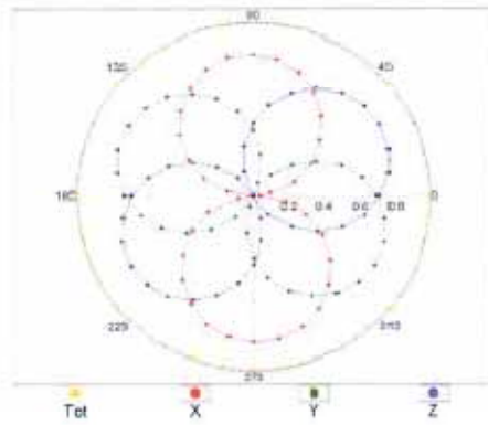
f=600 MHz,TEM
