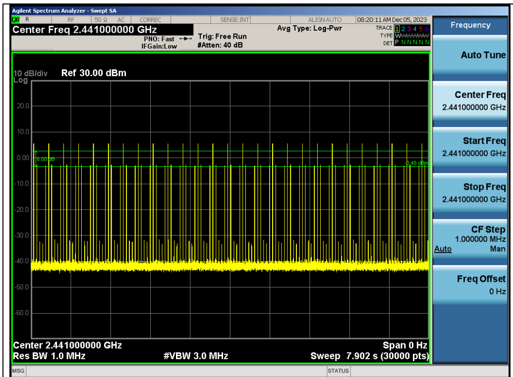
Test_Graph_GFSK_HOP_ANT1_NA_1Mbps_2441_Number of Burst
