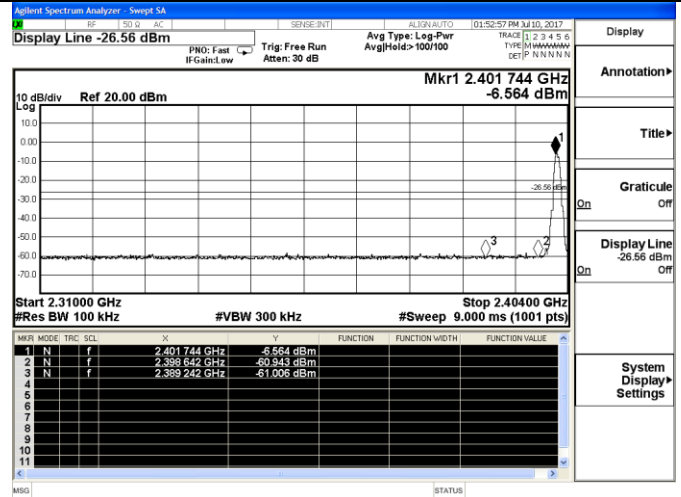
Channel 0 / 2402 MHz
