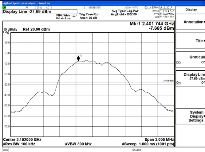
2401 – 2403 MHz
