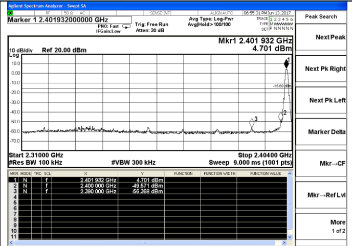
Channel 0 / 2402 MHz
