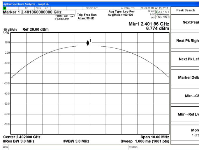
Channel 0 / 2402 MHz
