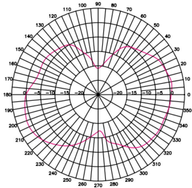
E-Plane Pattern @ 2.45GHz
