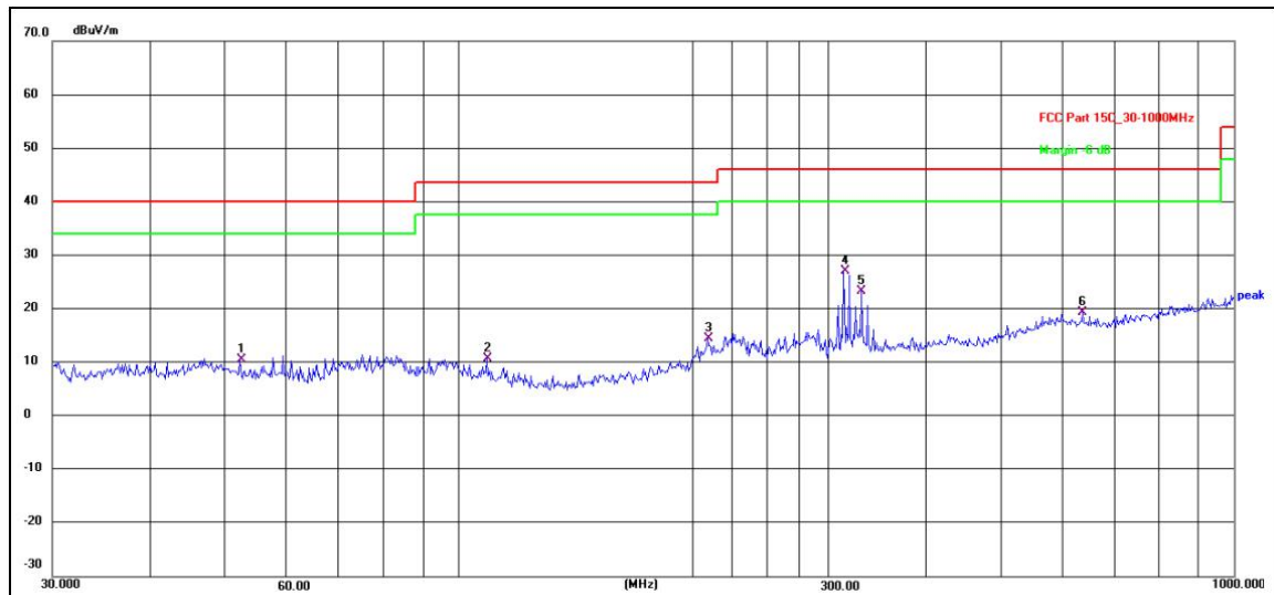
Test result for BT 2LE mode (Middle Channel)--External Antenna 1 Horizontal
