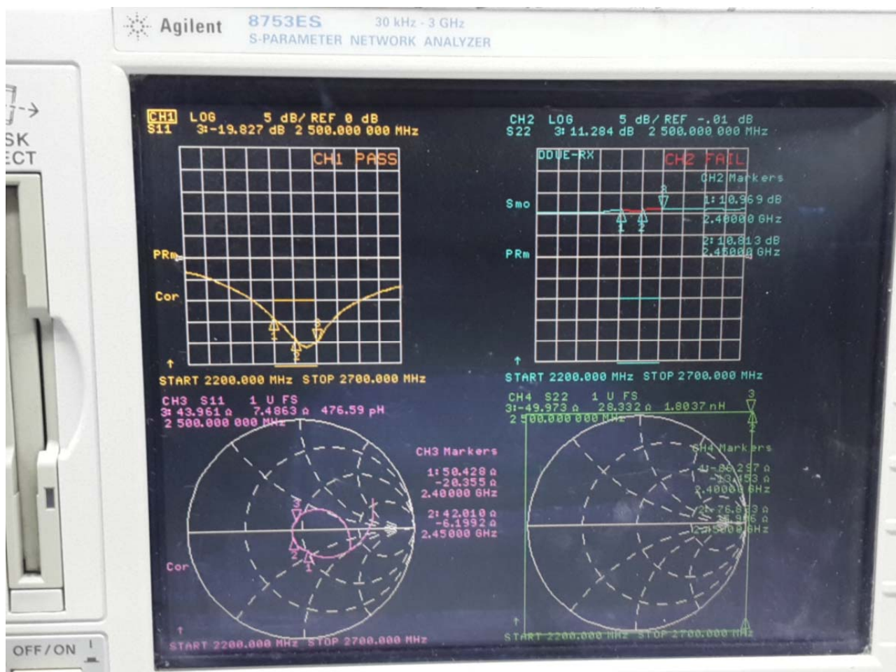
RF Antenna Assembly SPEC:2.4~2.5GHz
