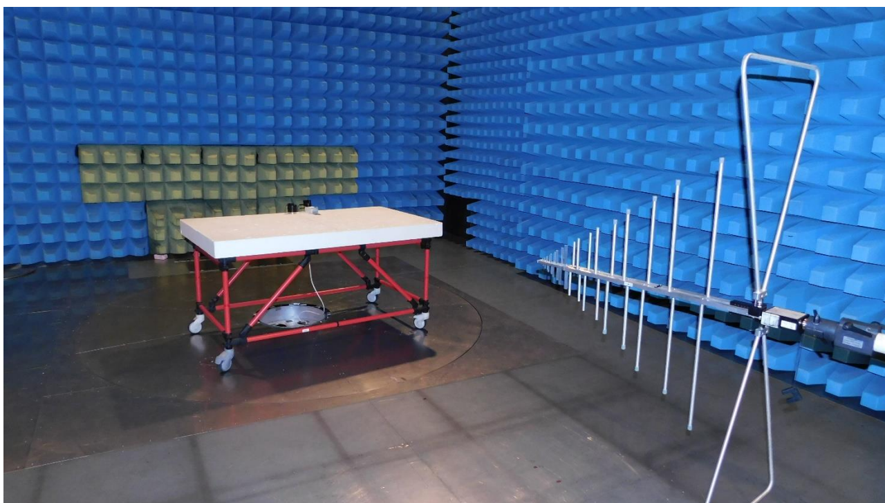
Picture 8: SAC, radiated emission test 30 MHz - 1 GHz (rear view), charging mode
