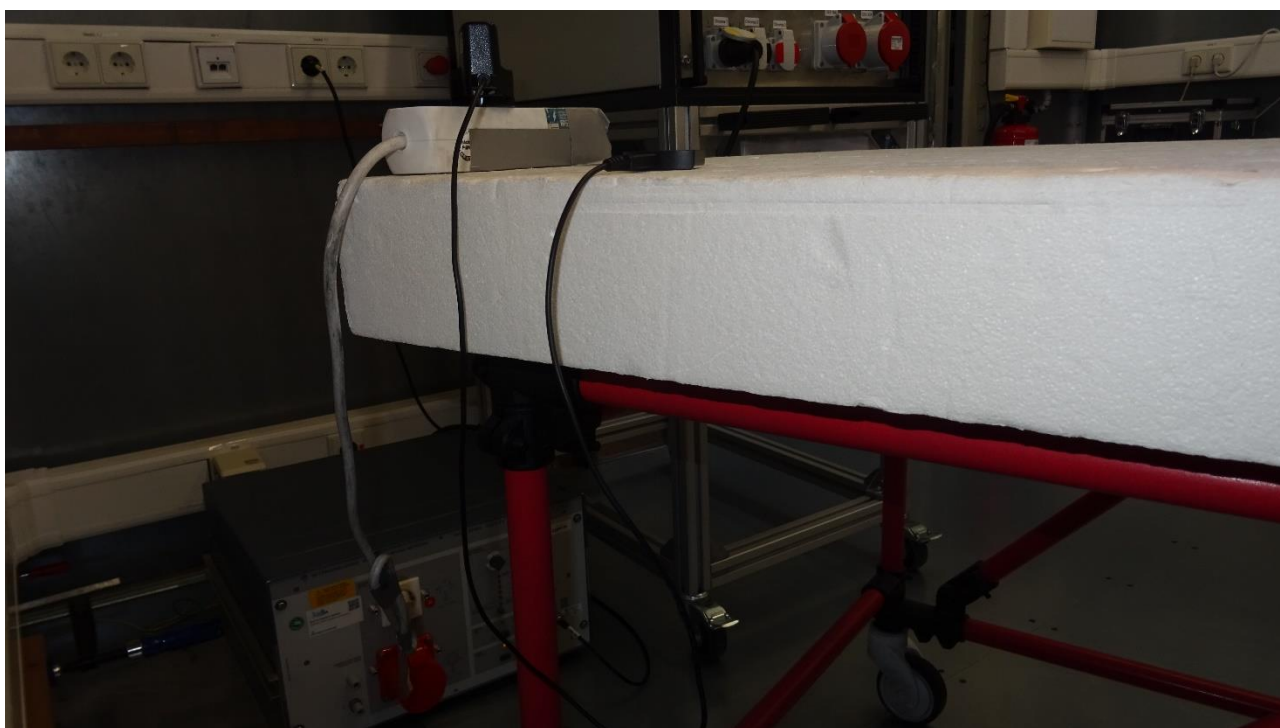
Picture 10: Test setup AC power line conducted emissions (rear view), standby mode
