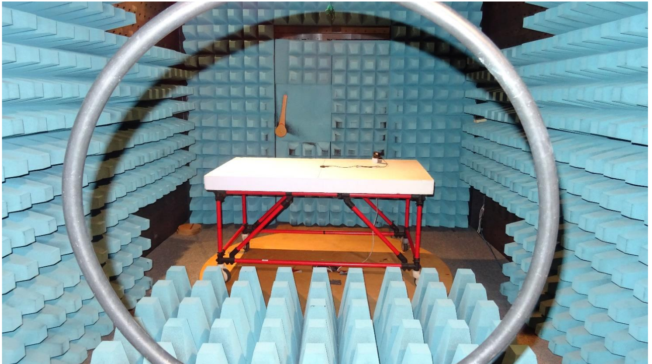
Picture 2: CDC, test setup radiated emission test 9 kHz - 30 MHz (rear view), standby mode
