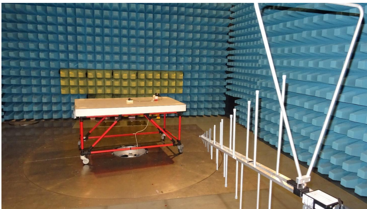
Picture 6: SAC, radiated emission test 30 MHz - 1 GHz (rear view), standby mode
