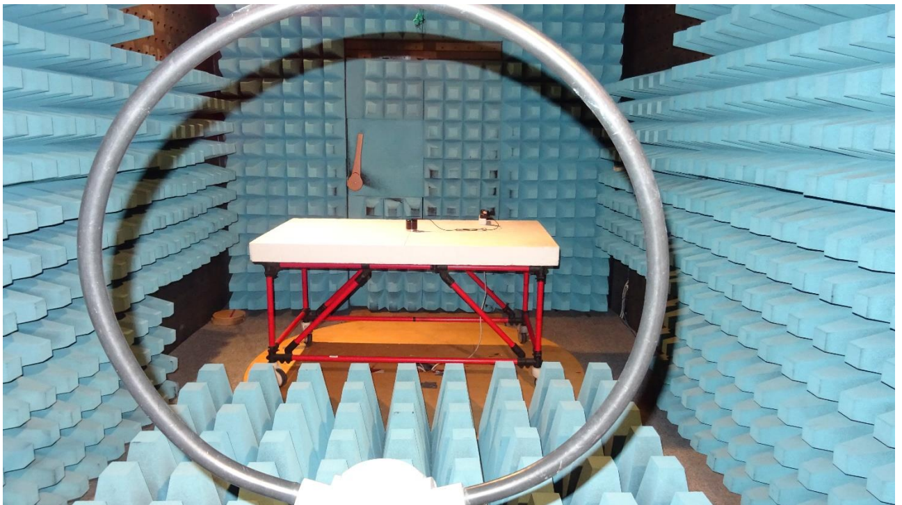
Picture 4: CDC, test setup radiated emission test 9 kHz - 30 MHz (rear view), charging mode
