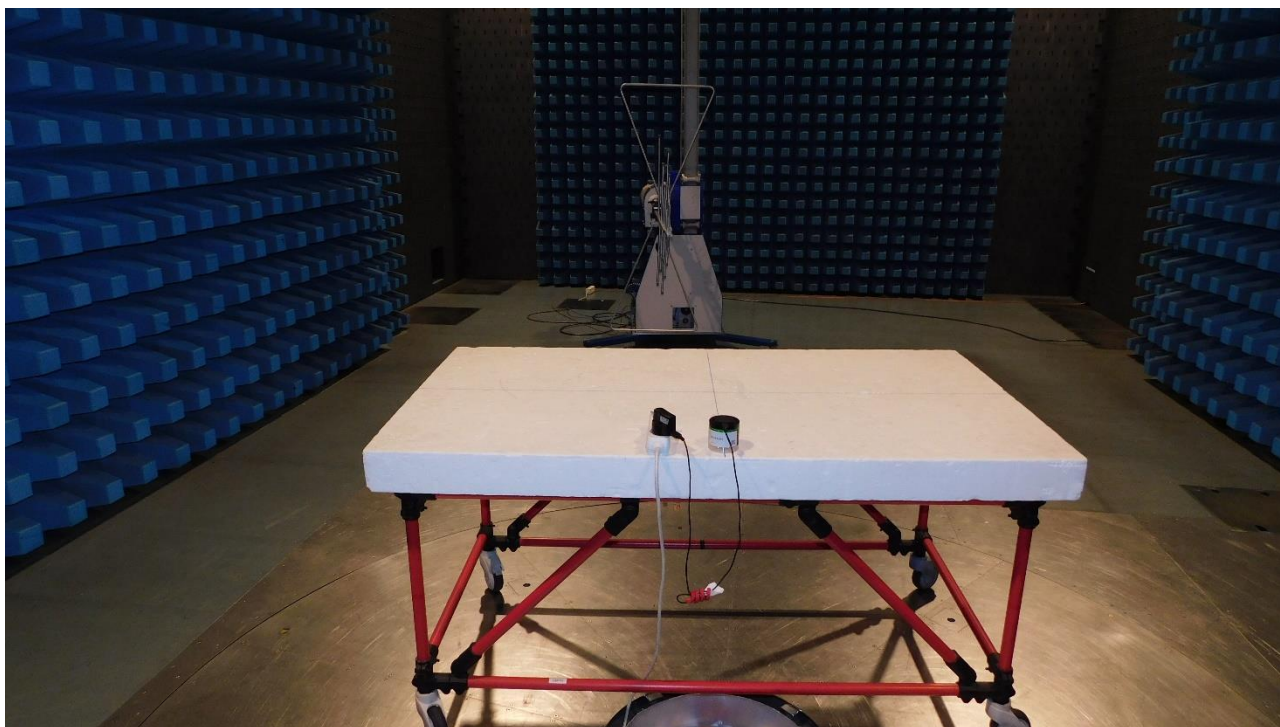
Picture 7: SAC, radiated emission test 30 MHz - 1 GHz (front view), charging mode
