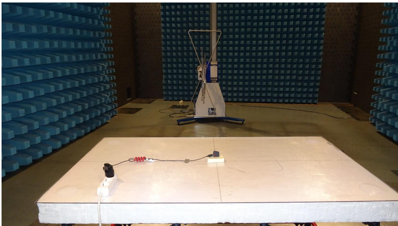
Picture 5: SAC, radiated emission test 30 MHz - 1 GHz (front view), standby mode
