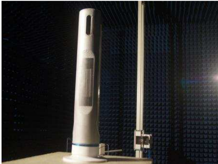
Photograph 4: Set-up for Radiated Spurious Emission (18GHz ~ 26GHz)
