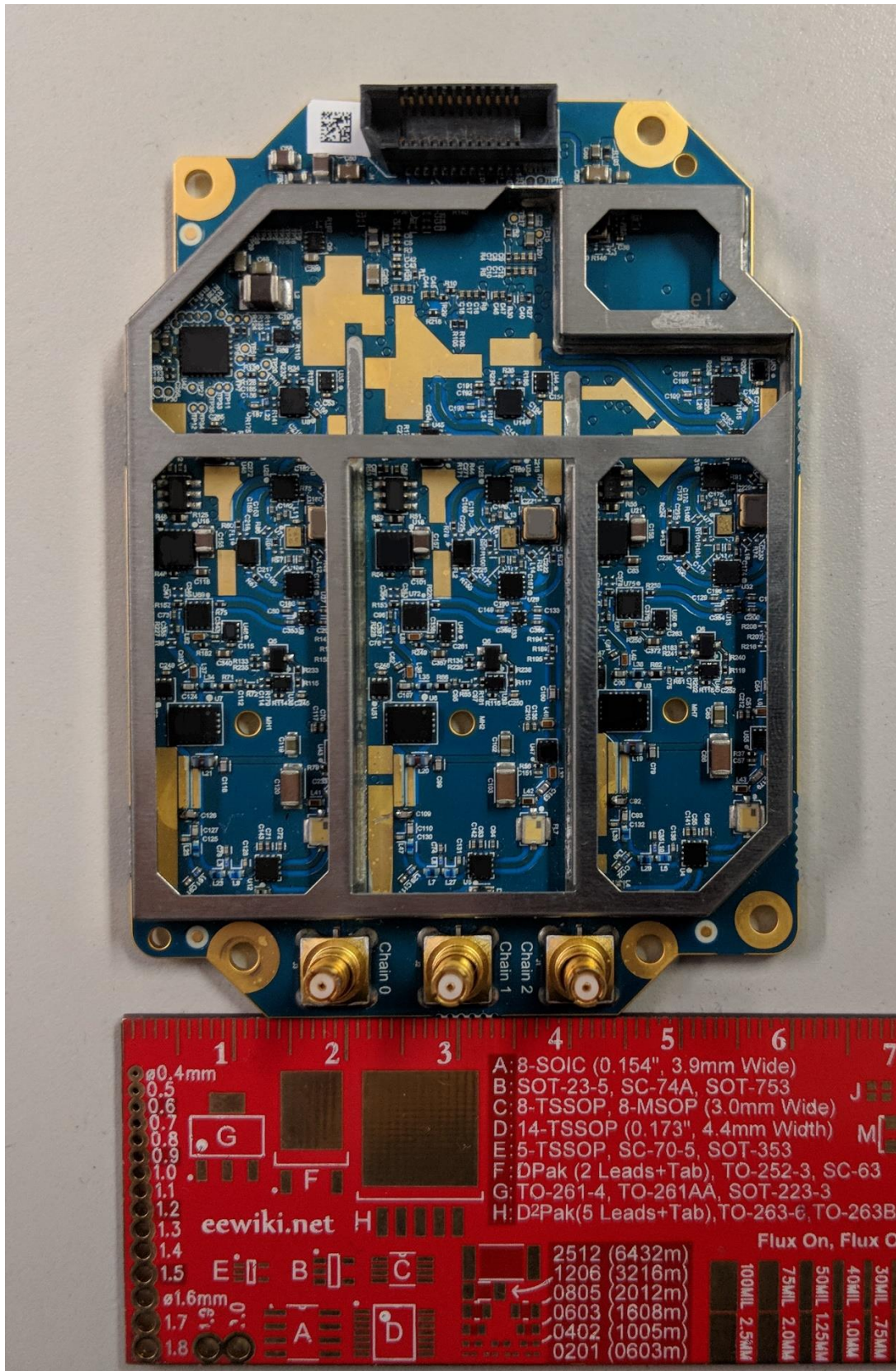
Picture 1: Front View w/o EMI Shield
