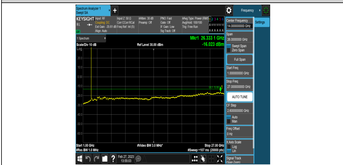
Band41-20MHz-256QAM-Lowest-E-TM3.1A-1000~27000
