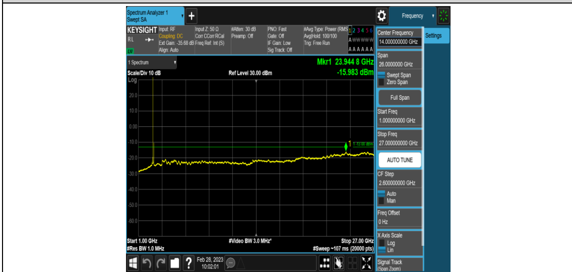
Band41-10MHz-256QAM-Middle-E-TM3.1A-1000~27000
