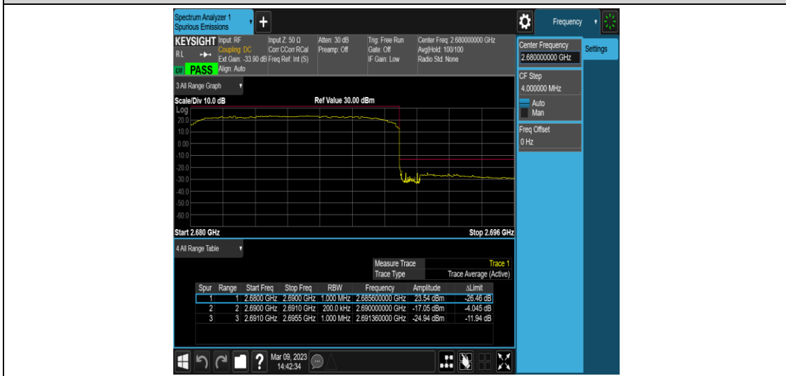
Band41-20MHz-256QAM-Highest-E-TM3.1A-2690.00~2691.00
