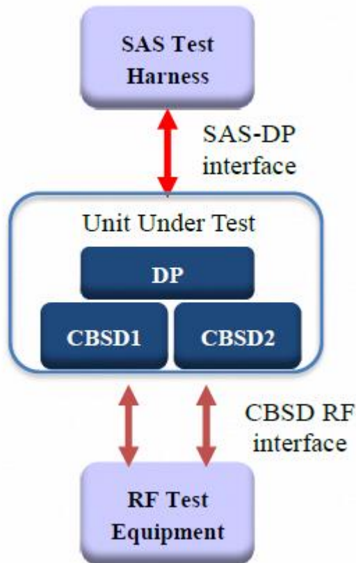
DP/CBSID as UUT, BTS-CBSID communication with Domain Proxy
