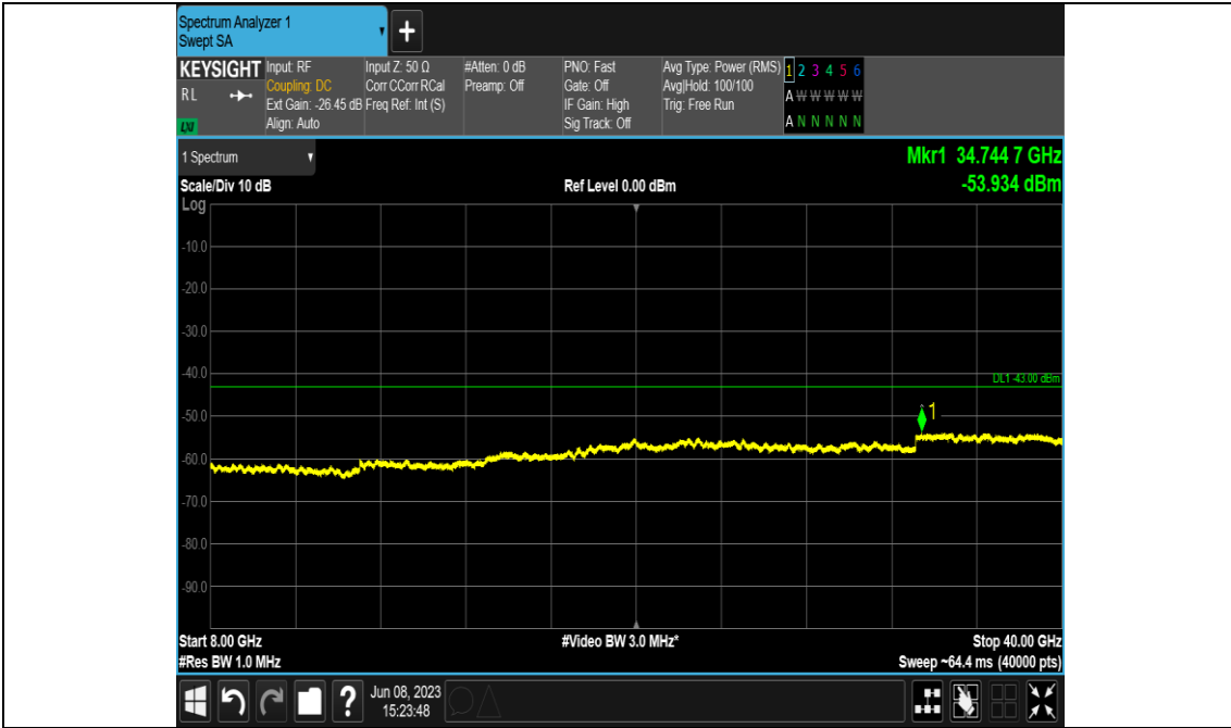
Band48-10MHz-256QAM-55990-E-TM3.1A-30~3530
