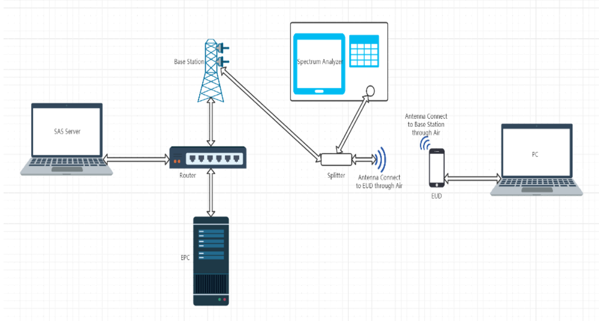
Test setup diagram for WINNF.PT.C.HBT Test case
