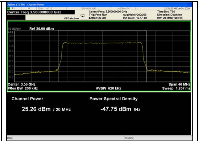
20MHz Full - Low CH 64QAM
