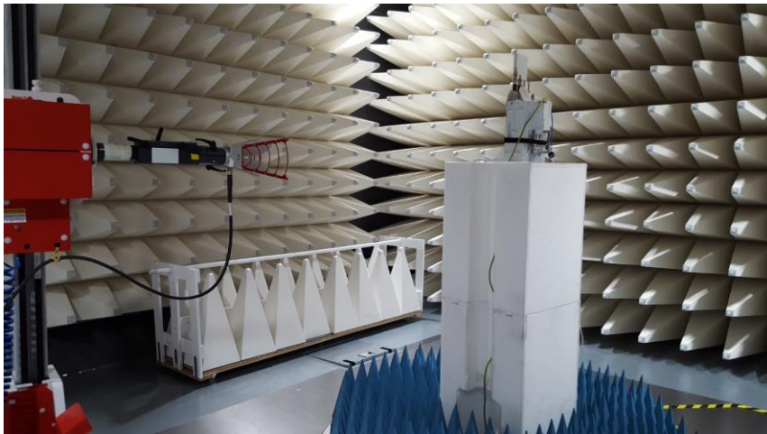
Figure B4. Radiated Setup 2
