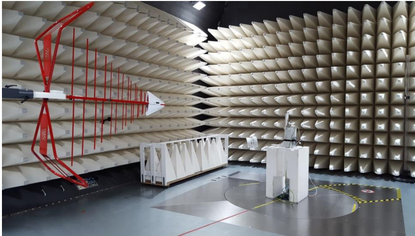
Figure B3. Radiated Setup 1
