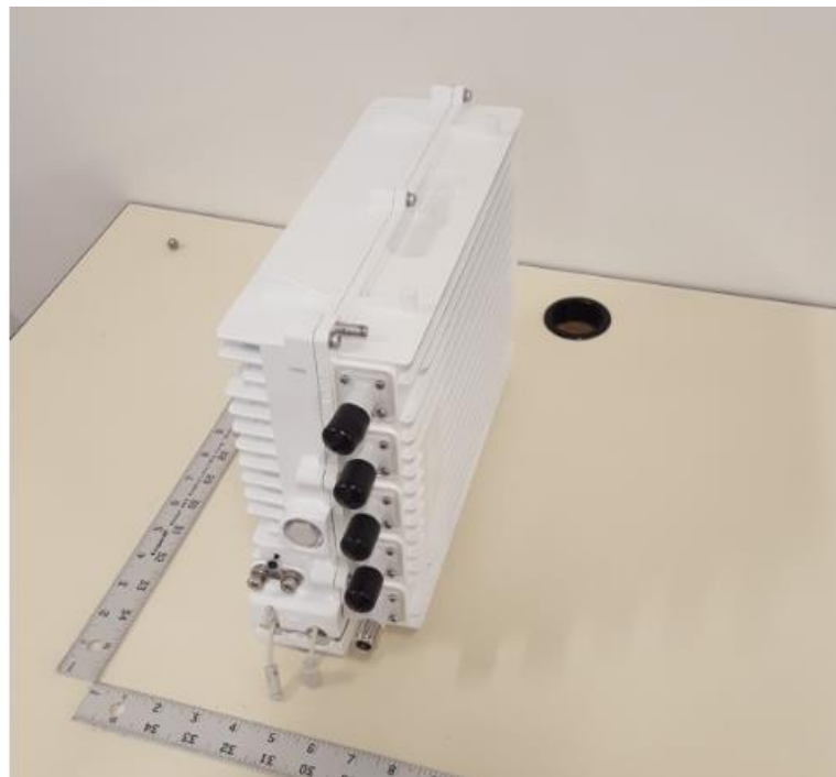
Figure B2. DUT Rear View
