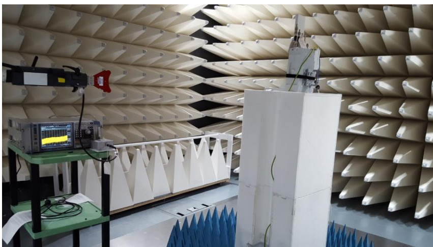
Figure B5. Radiated Setup 3
