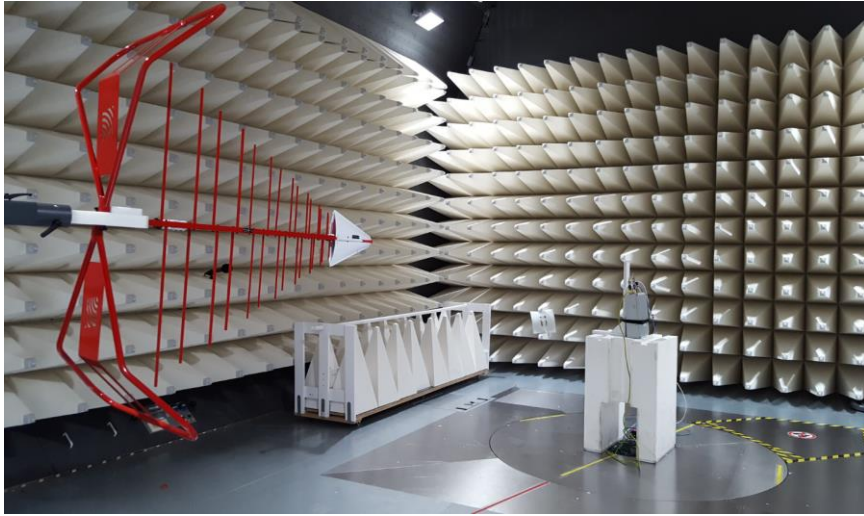
Figure B3. Radiated Setup 1
