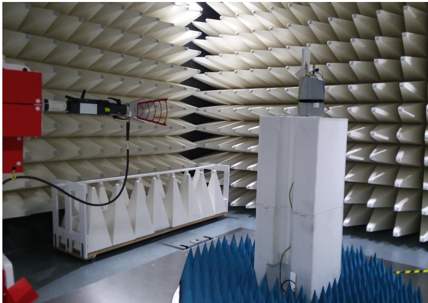
Figure B4. Radiated Setup 2
