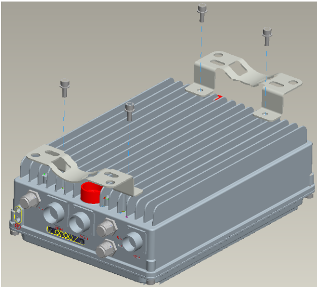
Figure 4-19 Install the Mounting Bracket
