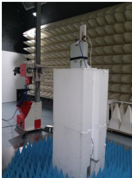
Figure B4. Radiated Setup 2
