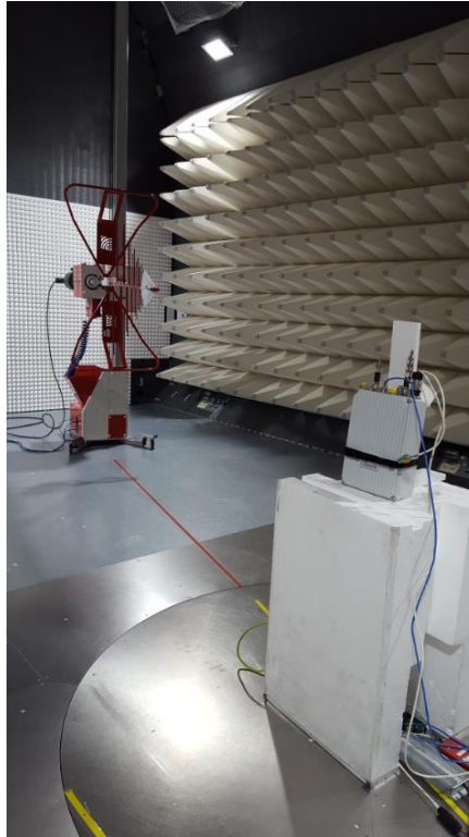
Figure B3. Radiated Setup 1
