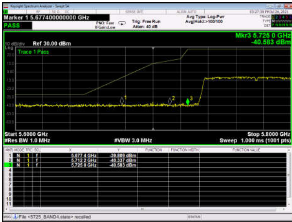
U-NII-3 ,Plot 1,Band Edge-802.11ac(80 MHz),5775MHz,Ant1 left side Bandedge
