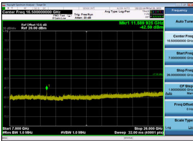
U-NII-3 ,Plot 4,7000MHz~26000MHz-802. 11ax(40MHz),5795MHz,Ant1
