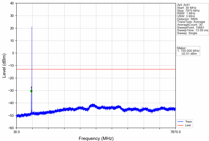
Band13_5MHz_16QAM_HCH_784.5MHz_RB_1_0_NTNV
