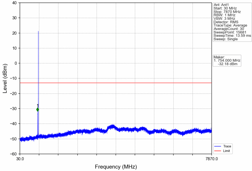
Band13_5MHz_QPSK_HCH_784.5MHz_RB_1_24_NTNV
