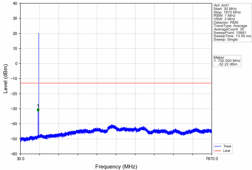
Band13_10MHz_16QAM_LCH_782MHz_RB_50_0_NTNV
