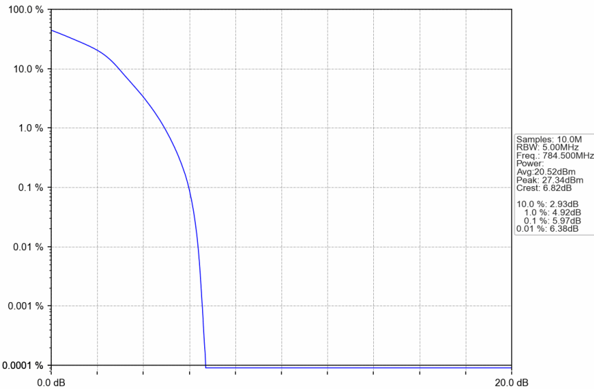
Band13_5MHz_16QAM_HCH_784.5MHz_RB_25_0_NTNV
