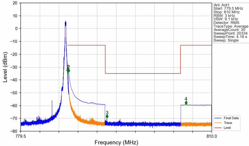
Band13_5MHz_16QAM_HCH_784.5MHz_RB_1_24_NTNV
