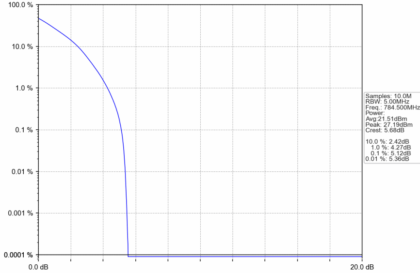
Band13_5MHz_QPSK_HCH_784.5MHz_RB_25_0_NTNV
