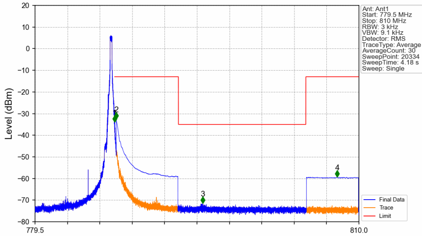
Band13_5MHz_QPSK_HCH_784.5MHz_RB_1_24_NTNV
