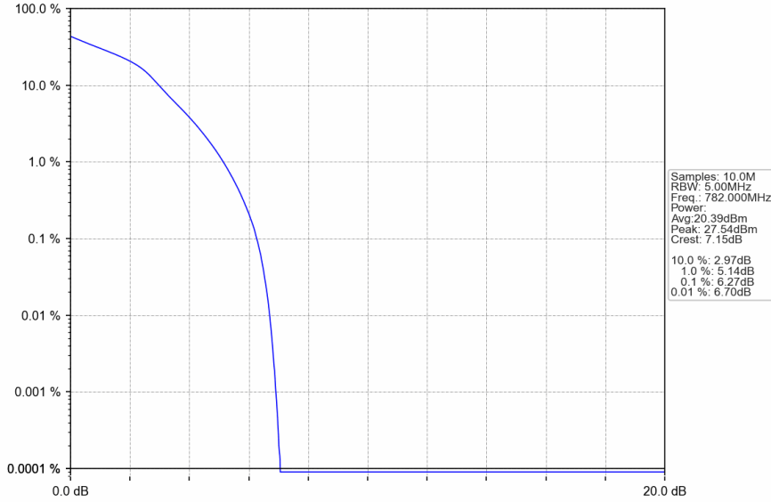
Band13_5MHz_16QAM_MCH_782MHz_RB_25_0_NTNV
