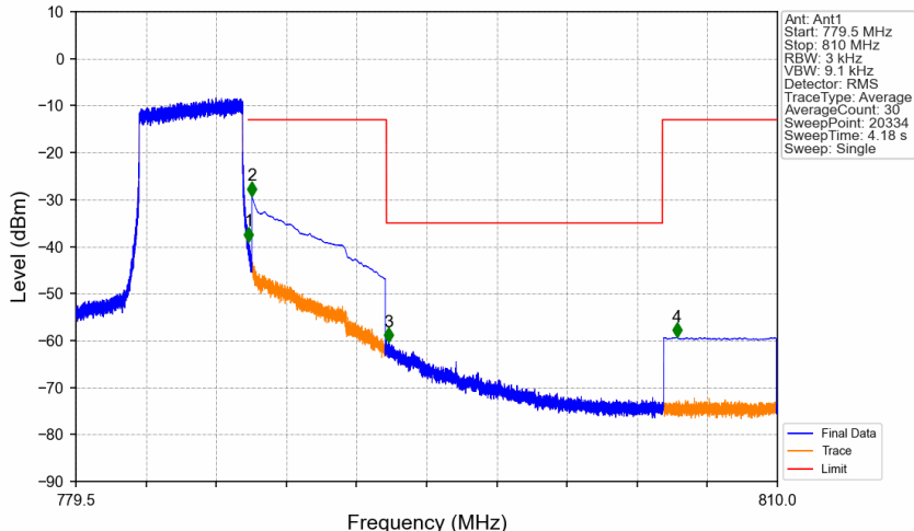
Band13_5MHz_16QAM_HCH_784.5MHz_RB_25_0_NTNV
