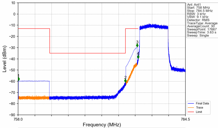
Band13_5MHz_16QAM_LCH_779.5MHz_RB_25_0_NTNV
