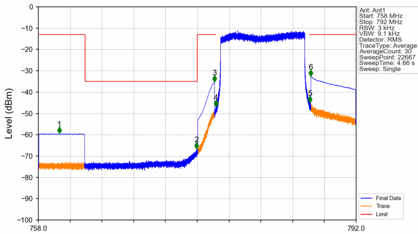
Band13_10MHz_16QAM_LCH_782MHz_RB_50_0_NTNV
