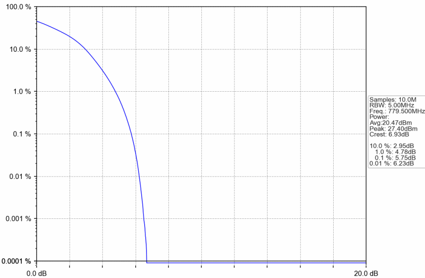
Band13_5MHz_16QAM_LCH_779.5MHz_RB_25_0_NTNV
