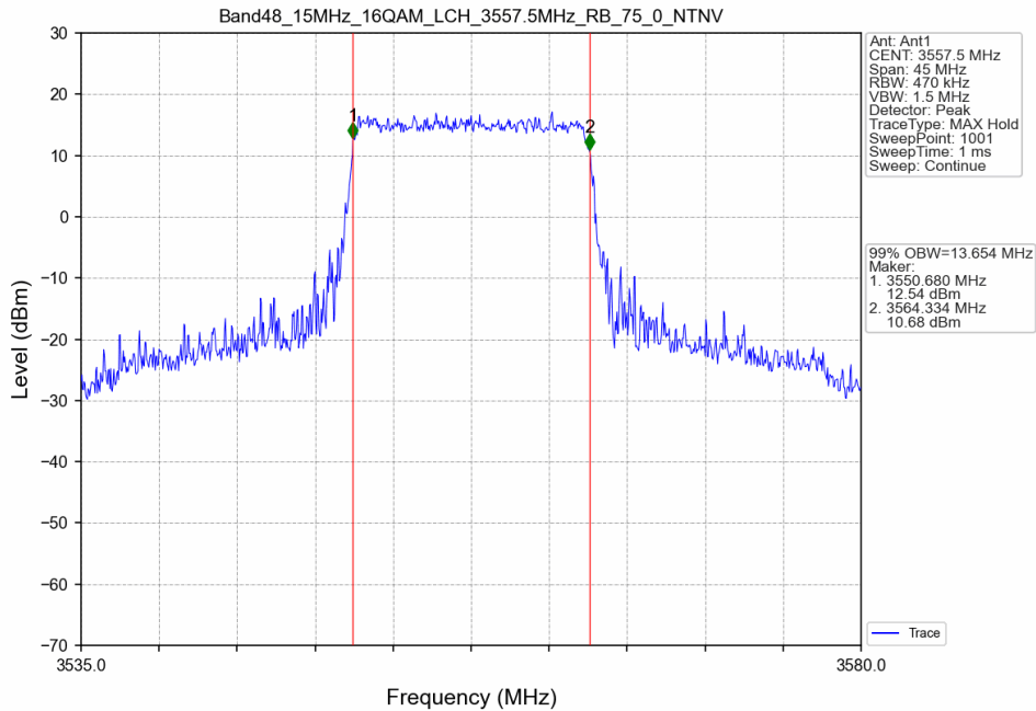
Band48_15MHz_16QAM_LCH_3557.5MHz_RB_75_0_NTNV
