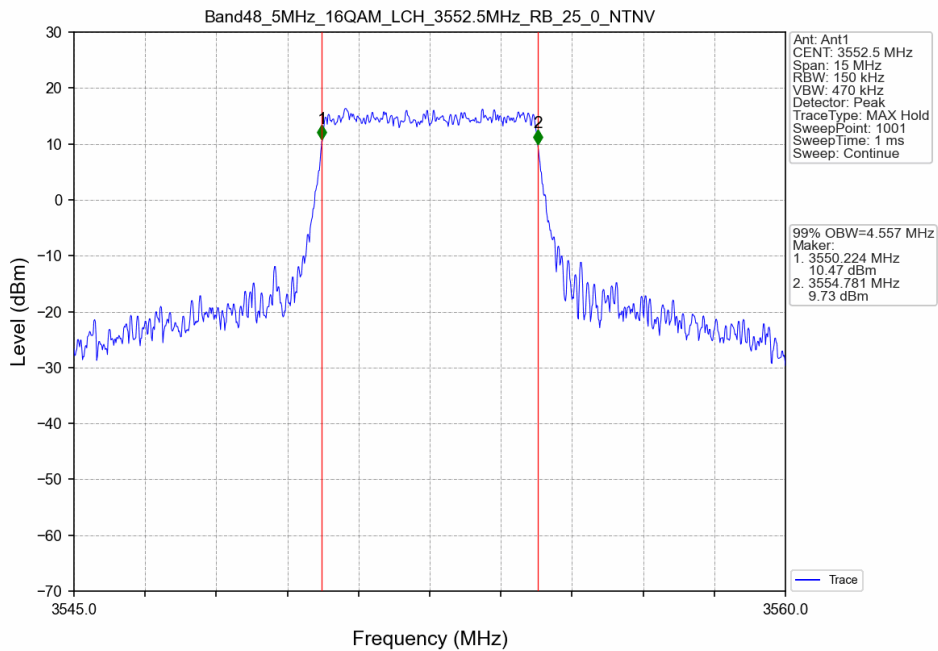
Band48_5MHz_16QAM_LCH_3552.5MHz_RB_25_0_NTNV
