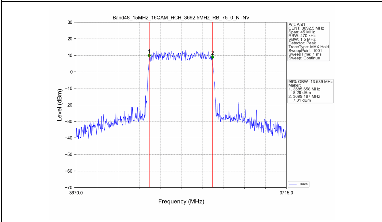
Band48_15MHz_16QAM_HCH_3692.5MHz_RB_75_0_NTNV
