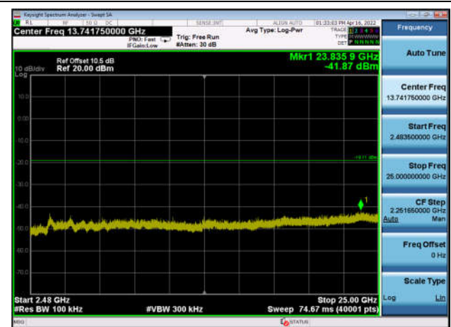
,Plot 4,2483.5MHz~25000MHz-802.11n(HT40),2452MHz,Ant1
