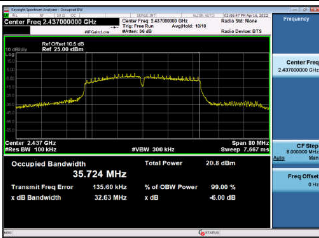
6dB Bandwidth-802.11n(HT40),2437MHz ,Ant1
