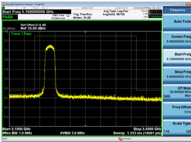
U-NII-1 ,802.11ac-VHT20, 5220MHz, Ant4
