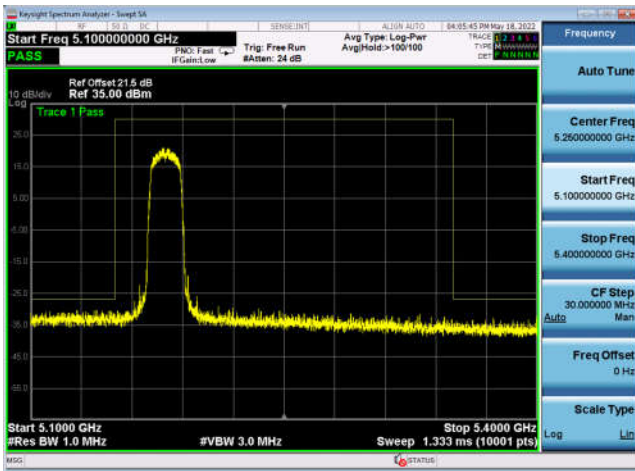
U-NII-1 ,802.11n-HT20, 5220MHz, Ant5
