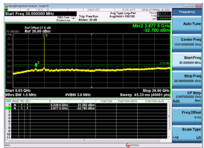
U-NII-1 ,802.11a, 5240MHz, Ant0
