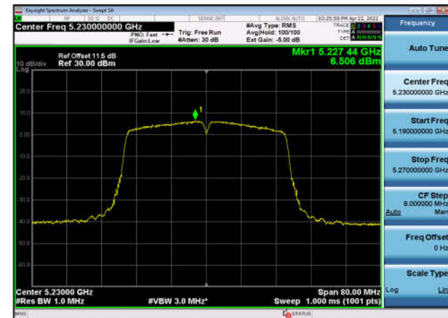
U-NII-1 Power spectral density-802.11 ac(40MHz),5230MHz,Ant1
