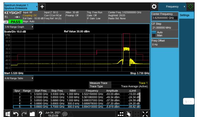
Highest channel
