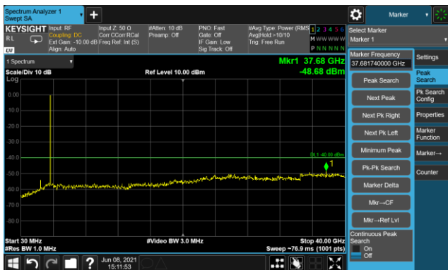
30MHz~40GHz
