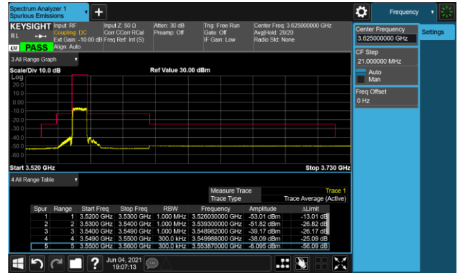
Lowest channel
