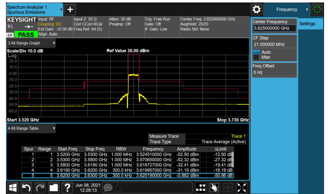
Middle channel
