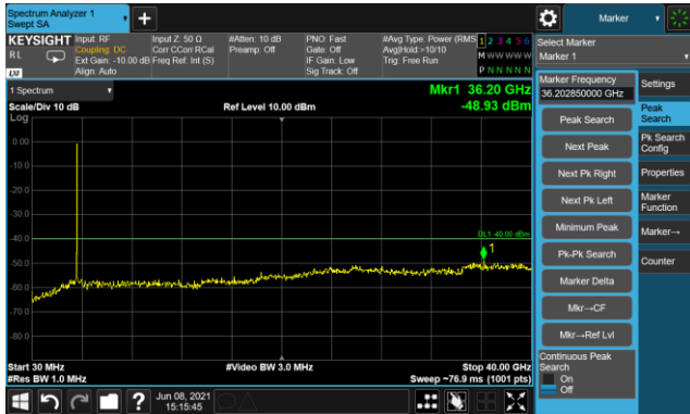
30MHz~40GHz
