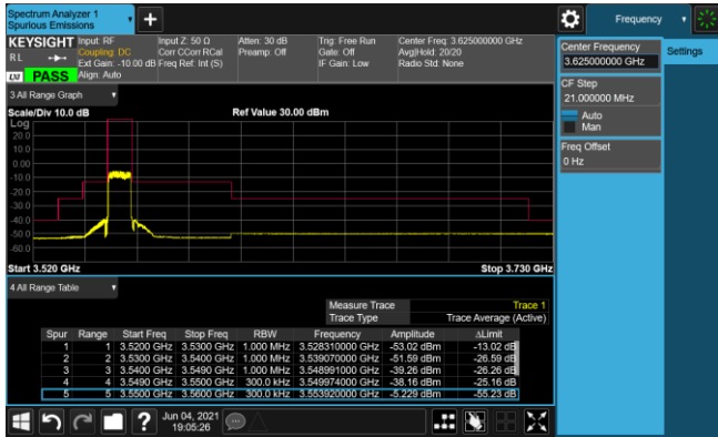
Lowest channel
