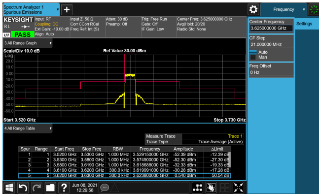
Middle channel
