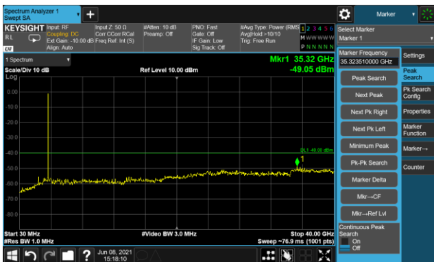
30MHz~40GHz
