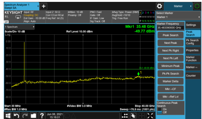
30MHz~40GHz
