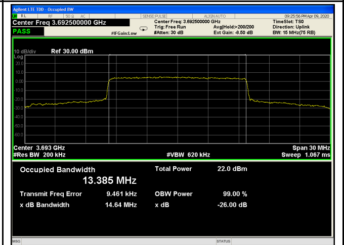
15MHz - High CH 16QAM
