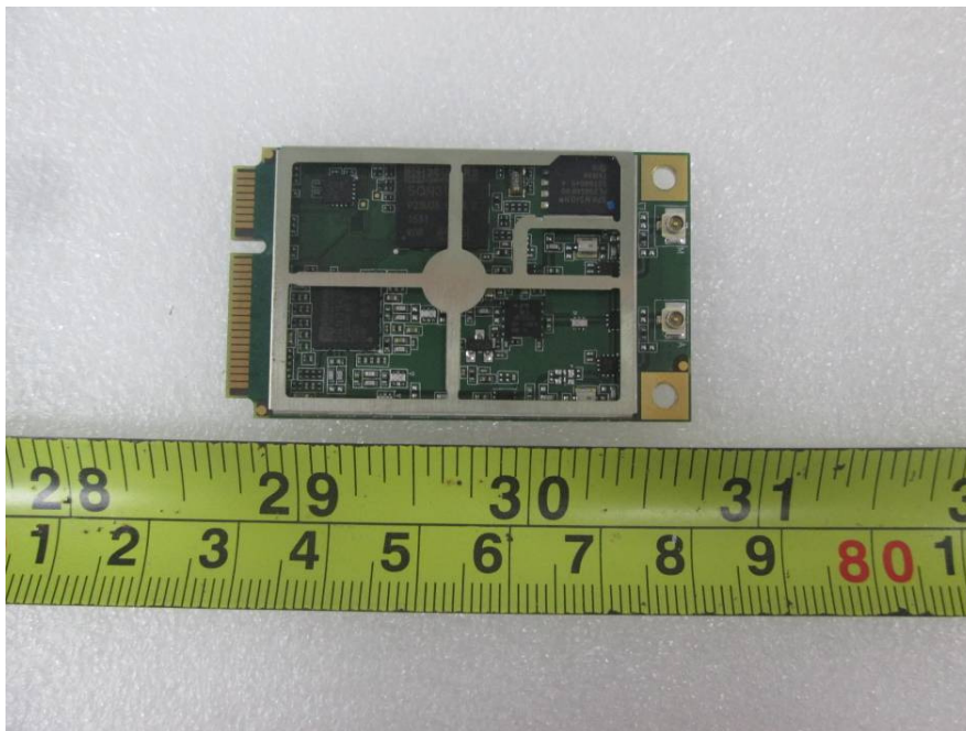
EUT – LTE Board Front View
