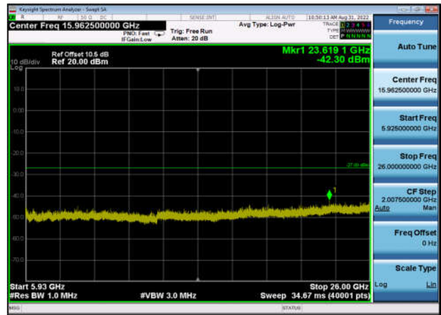
U-NII-3 ,Plot 3,5925MHz~26000MHz-802. 11ax(40MHz),5795MHz,Ant1
