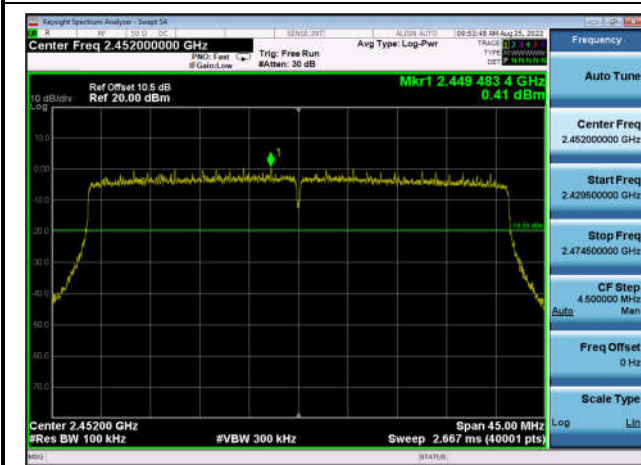
,Plot 1,Reference Level-802.11ax(HT40 ) ,2452MHz,Ant0
