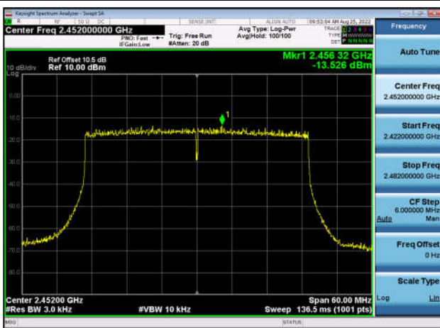
Power spectral density-802.11ax(HE40) ,2452MHz,Ant0
