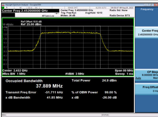
99% Bandwidth-802.11ax(HE40),2452MHz ,Ant0
