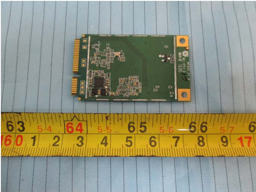
EUT –LTE Module Bottom Uncover View
