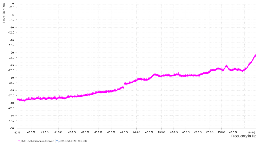
n261, Module0, 100MHz, 3CC, 64QAM, FULL RB, Middle channel, 40GHz-49.5GHz, V
