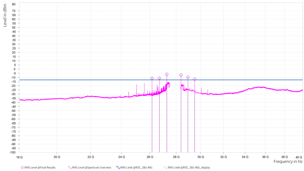
n261, Module0, 100MHz, 2CC, QPSK, FULL RB, Middle channel, 18GHz-40GHz, V
