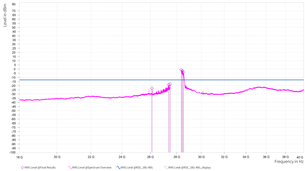
n261, Module0, 100MHz, 3CC, QPSK, FULL RB, High channel, 18GHz-40GHz, H
