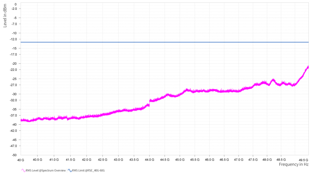
n261, Module0, 100MHz, 2CC, QPSK, FULL RB, Middle channel, 40GHz-49.5GHz, V
