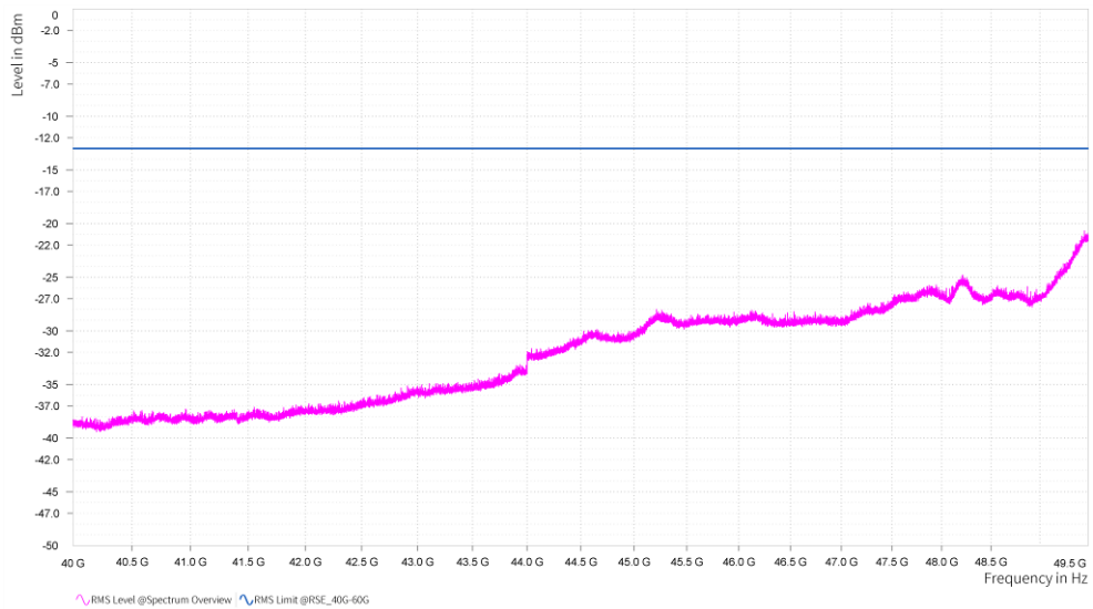
n261, Module0, 100MHz, 2CC, QPSK, FULL RB, High channel, 40GHz-49.5GHz, V
