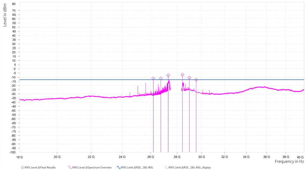
n261, Module0, 100MHz, 1CC, QPSK, FULL RB, Middle channel, 18GHz-40GHz, V
