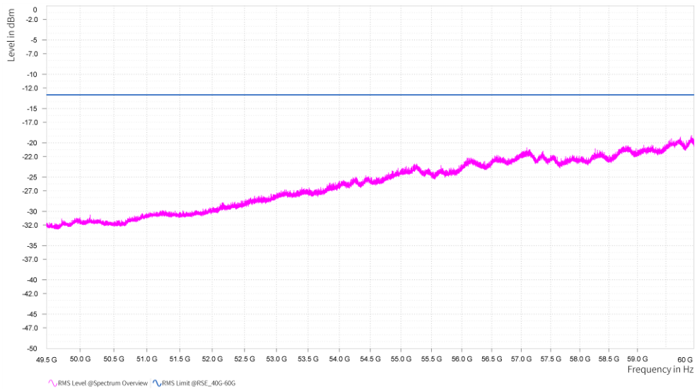
n261, Module0, 100MHz, 3CC, 64QAM, FULL RB, Low channel, 49.5GHz-60GHz, V
