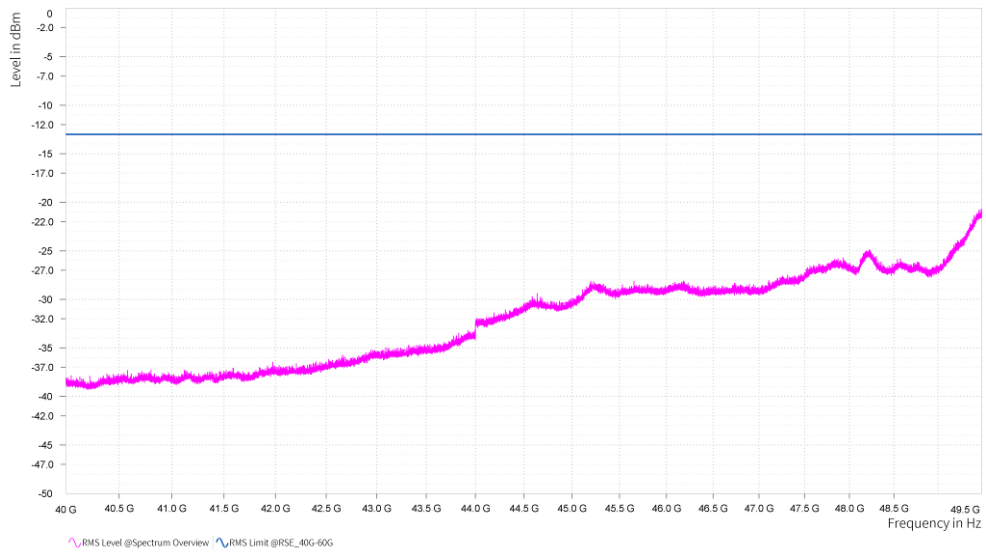
n261, Module0, 100MHz, 2CC, QPSK, FULL RB, Low channel, 40GHz-49.5GHz, H
