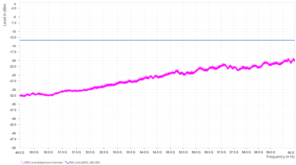
n261, Module0, 100MHz, 2CC, QPSK, FULL RB, Low channel, 49.5GHz-60GHz, V
