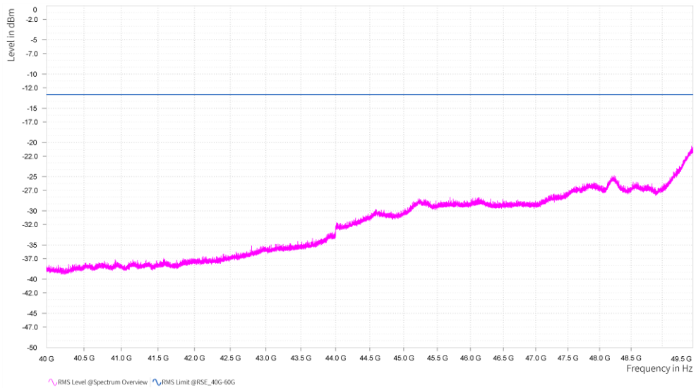
n261, Module0, 100MHz, 2CC, QPSK, FULL RB, Low channel, 40GHz-49.5GHz, V
