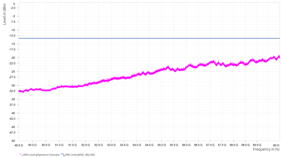
n261, Module0, 100MHz, 2CC, QPSK, FULL RB, Low channel, 49.5GHz-60GHz, H
