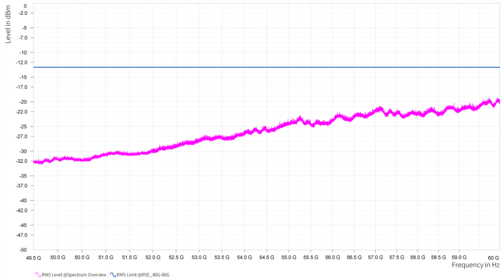
n261, Module0, 100MHz, 3CC, QPSK, FULL RB, Middle channel, 49.5GHz-60GHz, H
