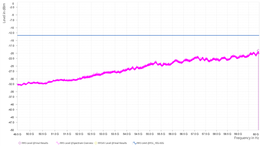
n261, Module0, 100MHz, 4CC, 64QAM, FULL RB, Low channel, 49.5GHz-60GHz, H
