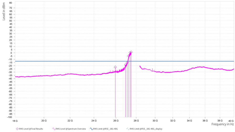
n261, Module0, 100MHz, 4CC, 64QAM, FULL RB, Low channel, 18GHz-40GHz, H
