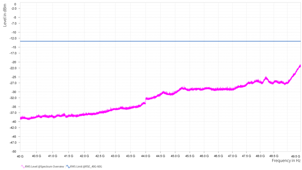
n261, Module0, 100MHz, 3CC, QPSK, FULL RB, High channel, 40GHz-49.5GHz, H
