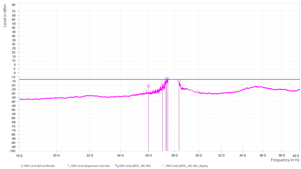
n261, Module0, 100MHz, 3CC, QPSK, FULL RB, Middle channel, 18GHz-40GHz, H
