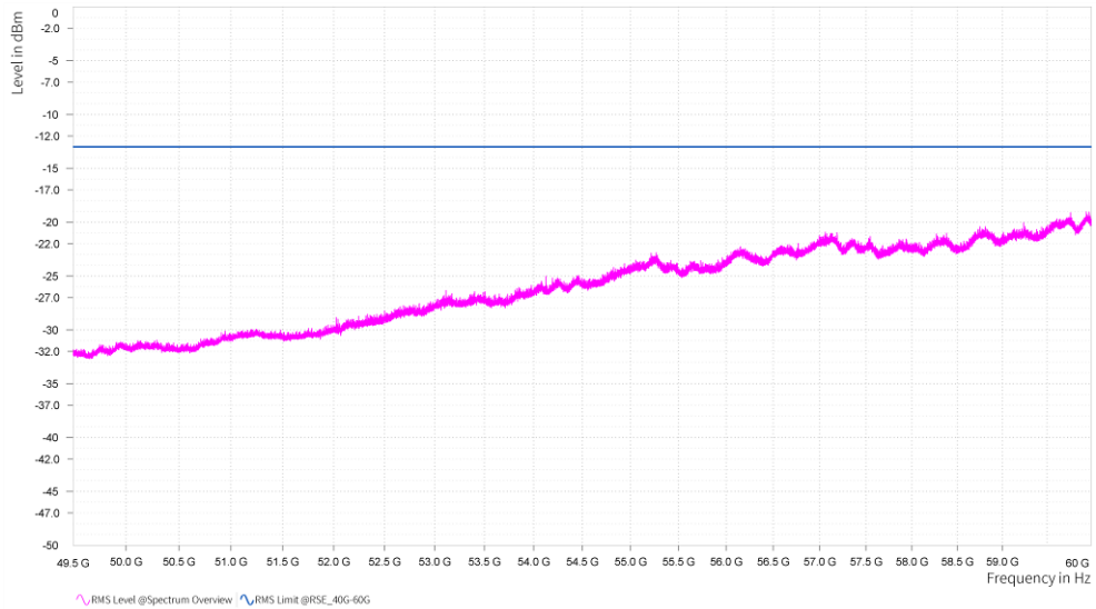
n261, Module0, 100MHz, 3CC, 64QAM, FULL RB, High channel, 49.5GHz-60GHz, V
