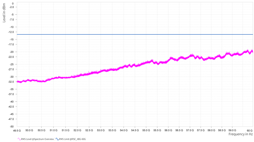
n261, Module0, 100MHz, 1CC, QPSK, FULL RB, High channel, 49.5GHz-60GHz, H
