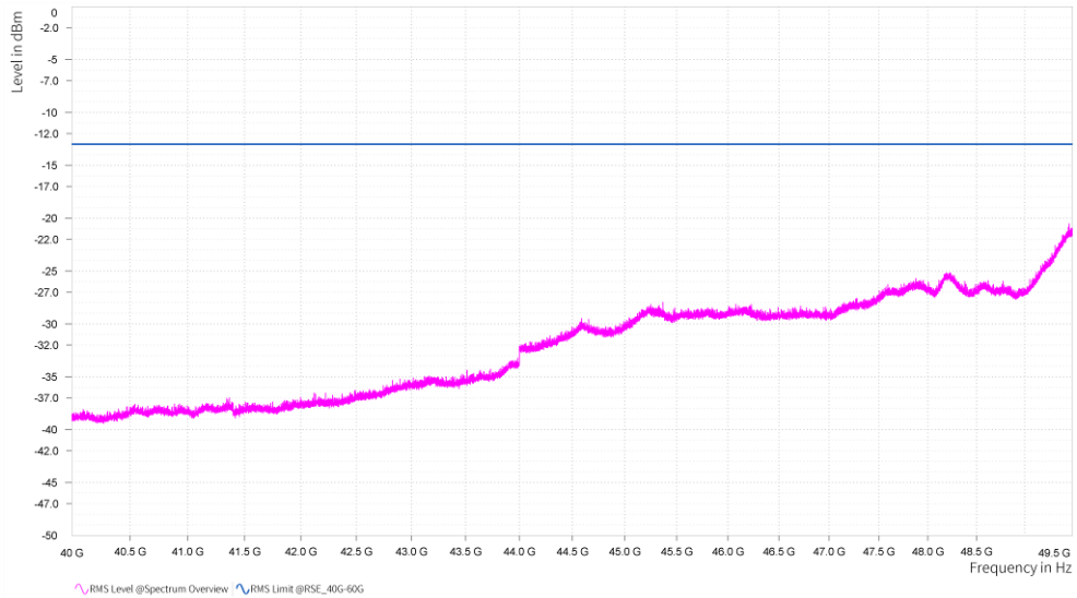
n261, Module0, 100MHz, 4CC, QPSK, FULL RB, Low channel, 40GHz-49.5GHz, V
