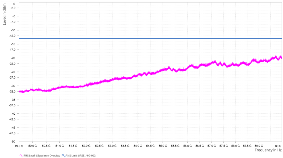
n261, Module0, 100MHz, 1CC, QPSK, FULL RB, High channel, 49.5GHz-60GHz, V
