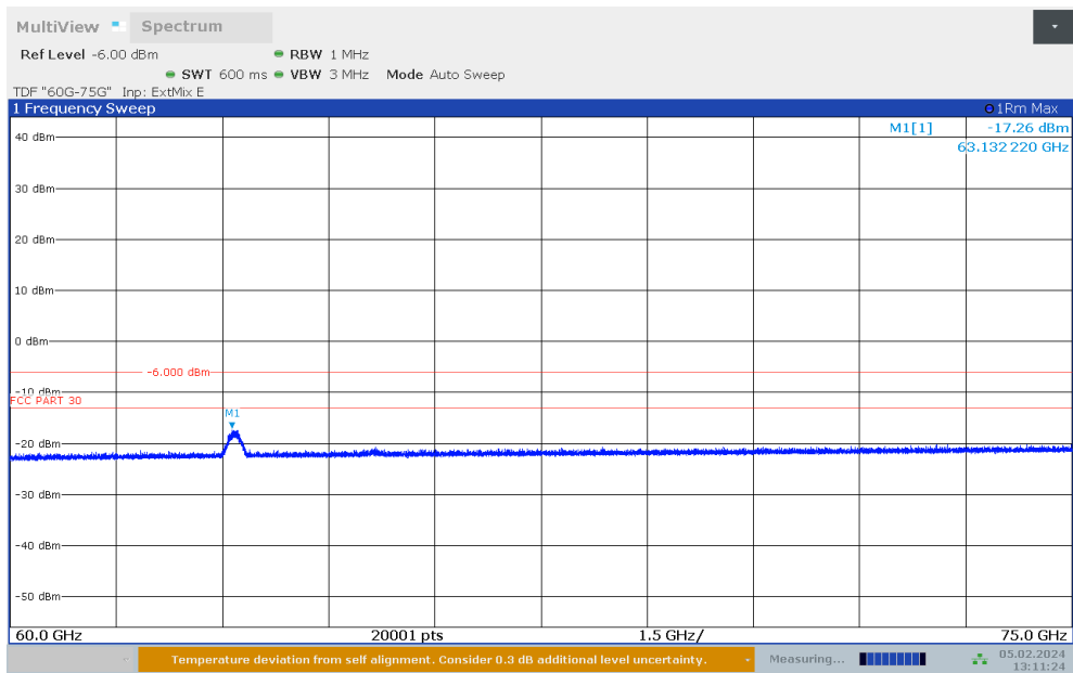
n261, Module0, 100MHz, 2CC, QPSK, FULL RB, Middle channel, 60GHz-75GHz, H
