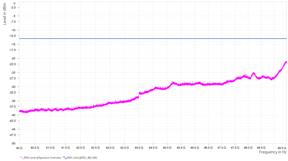
n261, Module0, 100MHz, 3CC, 64QAM, FULL RB, Low channel, 40GHz-49.5GHz, V
