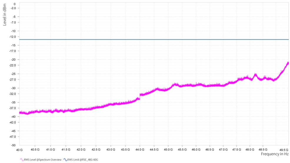
n261, Module0, 100MHz, 2CC, QPSK, FULL RB, High channel, 40GHz-49.5GHz, H
