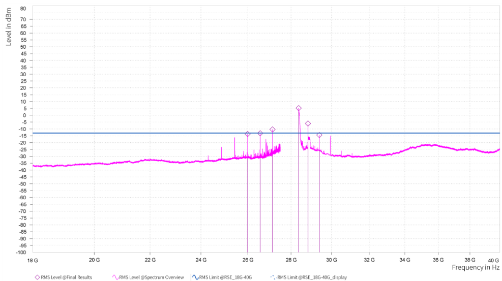
n261, Module0, 100MHz, 1CC, QPSK, FULL RB, High channel, 18GHz-40GHz, V
