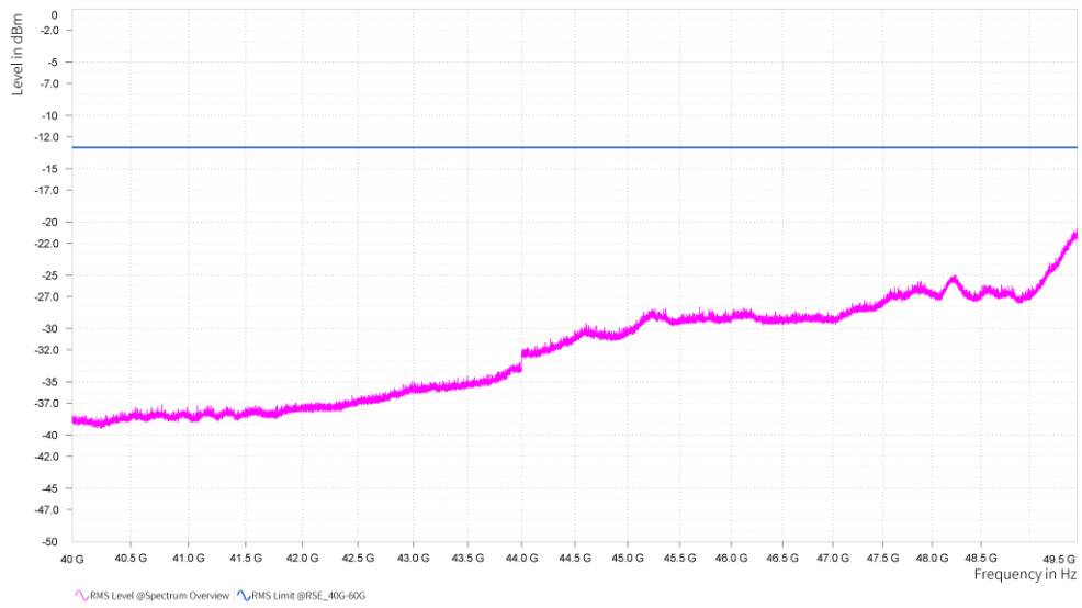
n261, Module0, 100MHz, 3CC, QPSK, FULL RB, Low channel, 40GHz-49.5GHz, H
