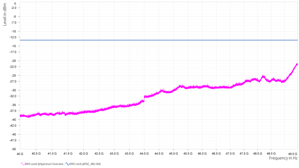
n261, Module0, 100MHz, 1CC, QPSK, FULL RB, Middle channel, 40GHz-49.5GHz, V
