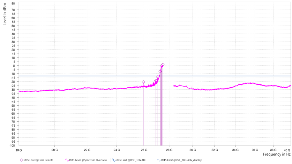
n261, Module0, 100MHz, 3CC, QPSK, FULL RB, Low channel, 18GHz-40GHz, H
