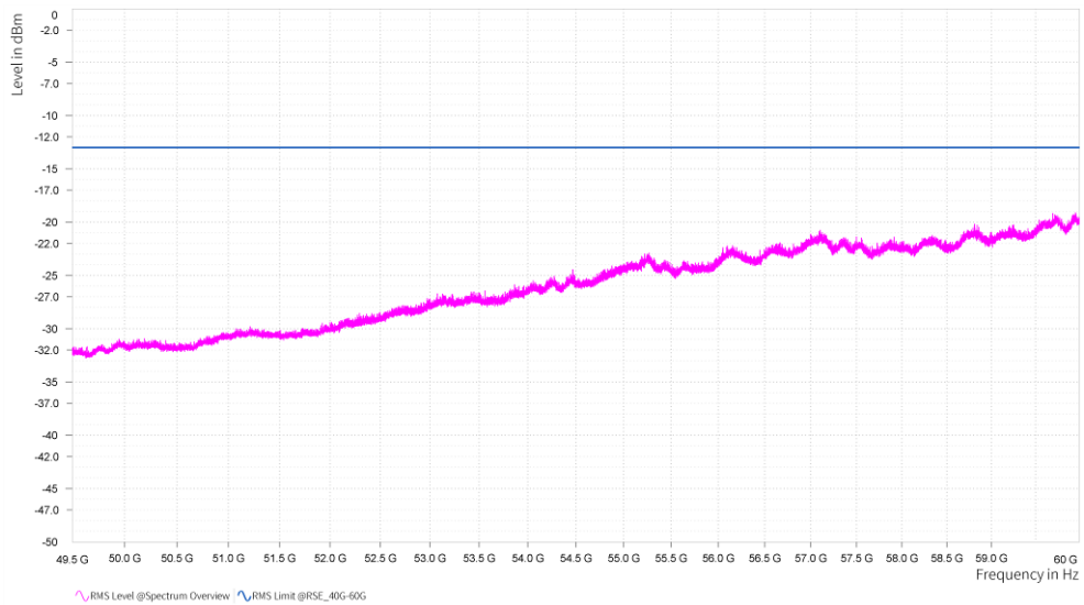
n261, Module0, 100MHz, 4CC, QPSK, FULL RB, Low channel, 49.5GHz-60GHz, V
