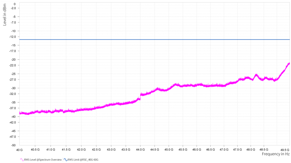
n261, Module0, 100MHz, 4CC, 64QAM, FULL RB, Low channel, 40GHz-49.5GHz, H
