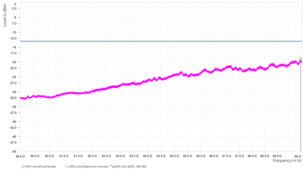
n261, Module0, 100MHz, 3CC, QPSK, FULL RB, Low channel, 49.5GHz-60GHz, H
