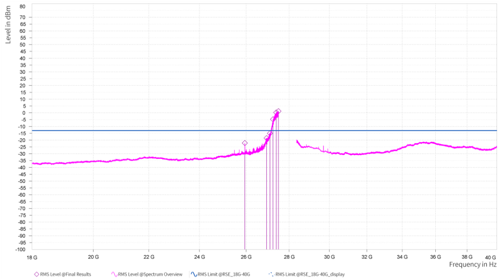
n261, Module0, 100MHz, 4CC, QPSK, FULL RB, Low channel, 18GHz-40GHz, V
