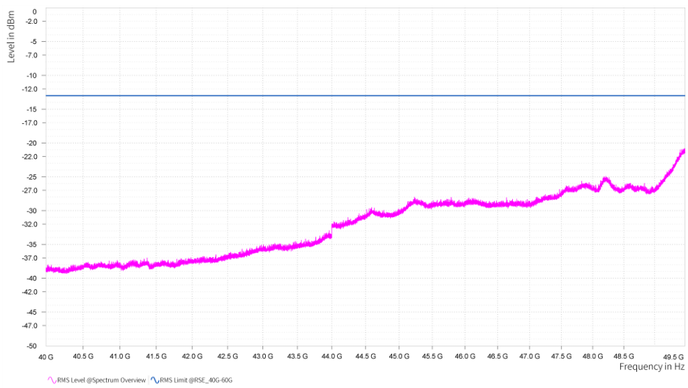
n261, Module0, 100MHz, 1CC, QPSK, FULL RB, Middle channel, 40GHz-49.5GHz, H
