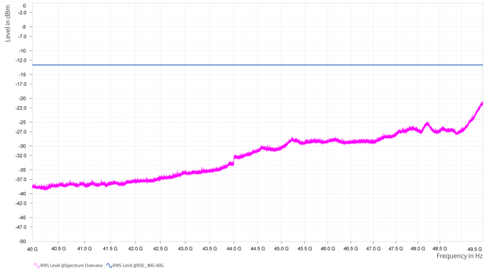
n261, Module0, 100MHz, 1CC, QPSK, FULL RB, High channel, 40GHz-49.5GHz, H
