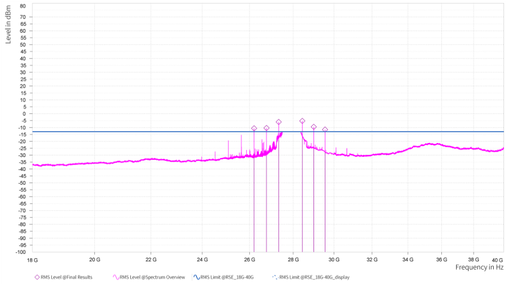
n261, Module0, 100MHz, 3CC, 64QAM, FULL RB, Middle channel, 18GHz-40GHz, V
