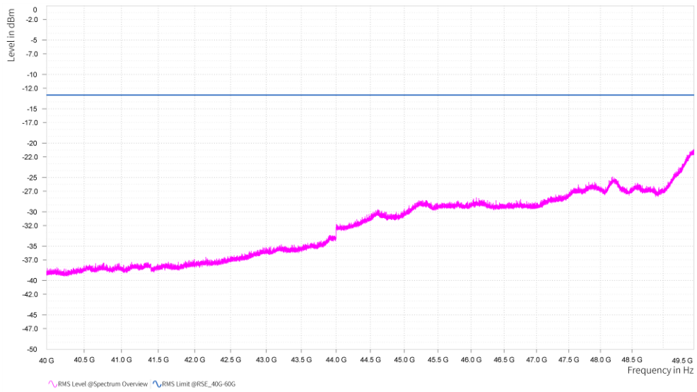
n261, Module0, 100MHz, 3CC, QPSK, FULL RB, Middle channel, 40GHz-49.5GHz, H
