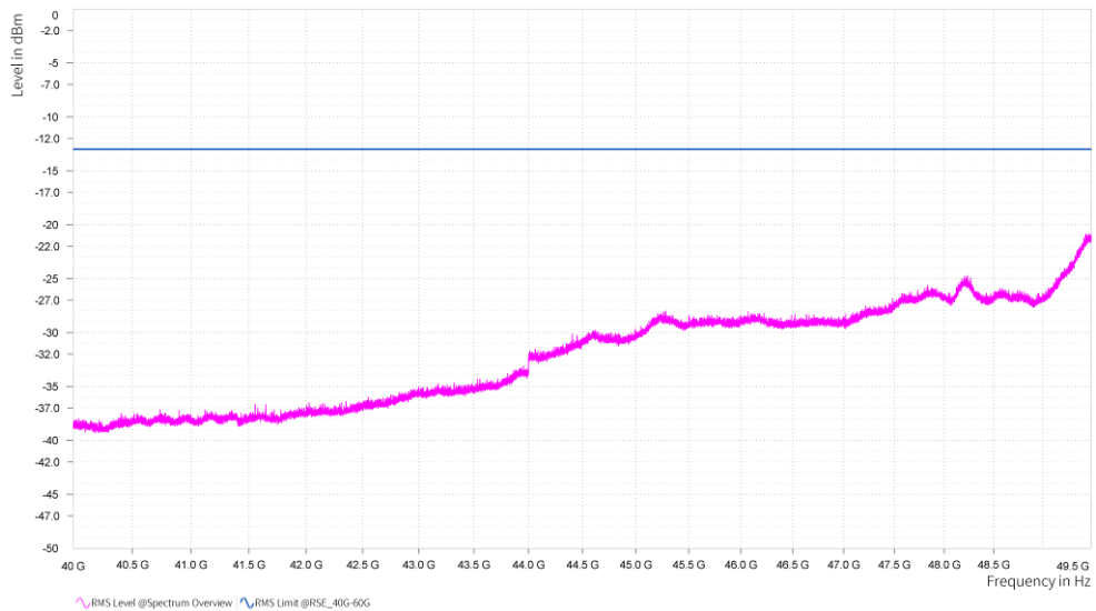
n261, Module0, 100MHz, 2CC, QPSK, FULL RB, Middle channel, 40GHz-49.5GHz, H
