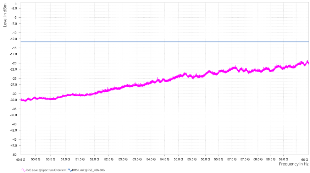
n261, Module0, 100MHz, 1CC, QPSK, FULL RB, Middle channel, 49.5GHz-60GHz, H
