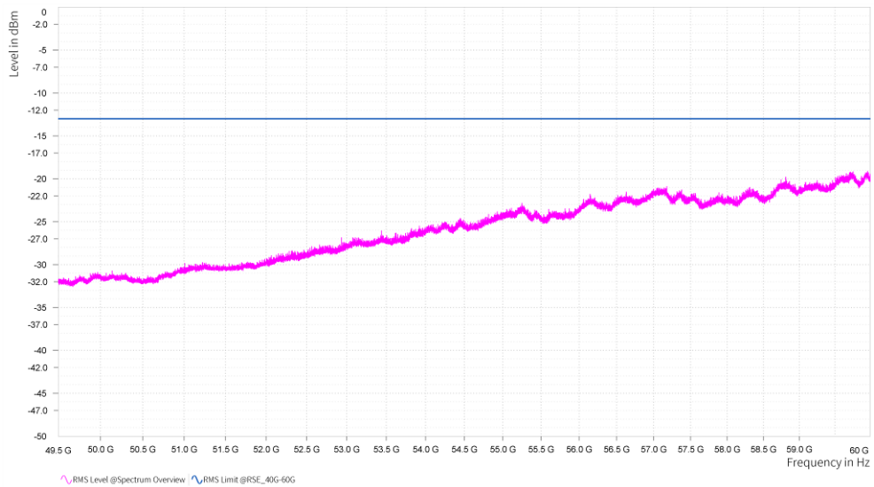
n261, Module0, 100MHz, 2CC, QPSK, FULL RB, Middle channel, 49.5GHz-60GHz, H
