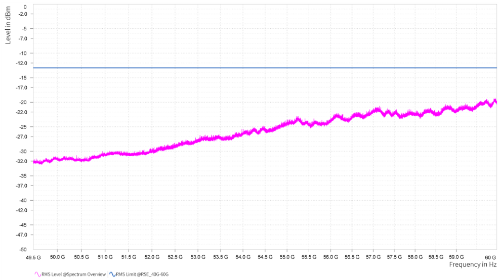
n261, Module0, 100MHz, 3CC, QPSK, FULL RB, High channel, 49.5GHz-60GHz, H
