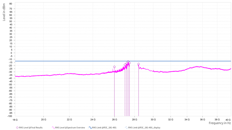
n261, Module0, 100MHz, 2CC, QPSK, FULL RB, Middle channel, 18GHz-40GHz, H
