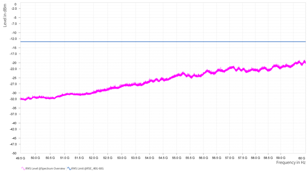
n261, Module0, 100MHz, 2CC, QPSK, FULL RB, Middle channel, 49.5GHz-60GHz, V
