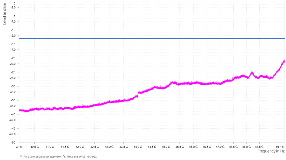
n261, Module0, 100MHz, 1CC, QPSK, FULL RB, High channel, 40GHz-49.5GHz, V
