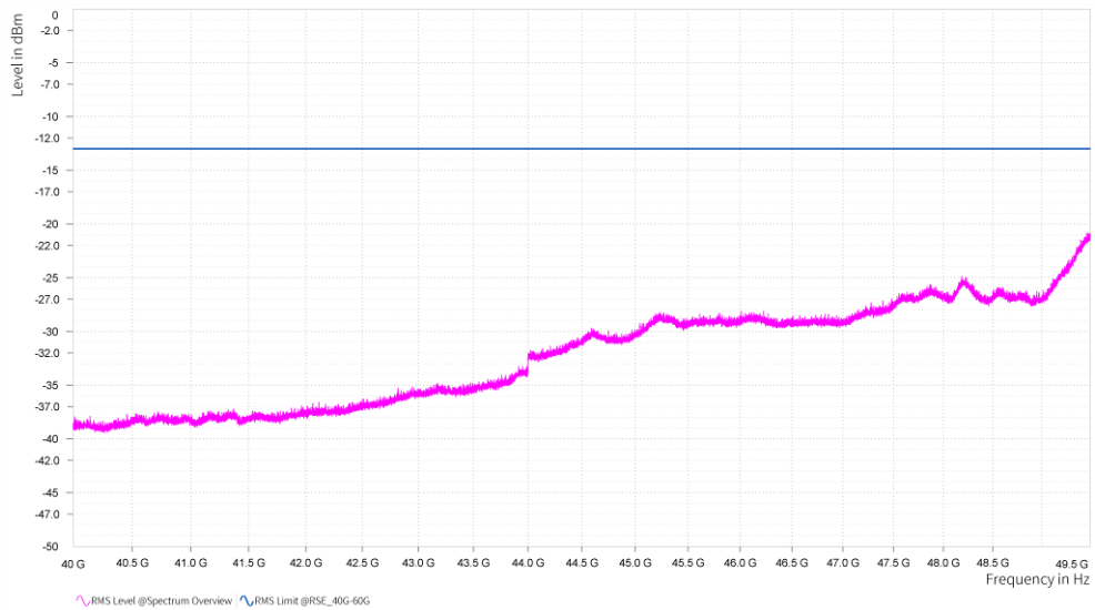
n261, Module0, 100MHz, 3CC, 64QAM, FULL RB, High channel, 40GHz-49.5GHz, V
