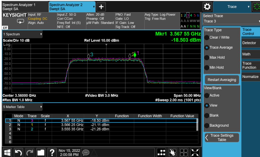
Port 0 and 1, 20MHz, bottom channel, QPSK, conducted PSD(dbm/MHz)
