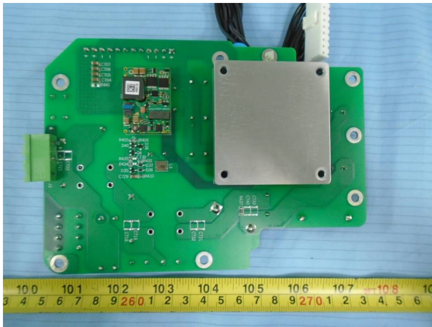
EUT –Power Main Board Bottom View
