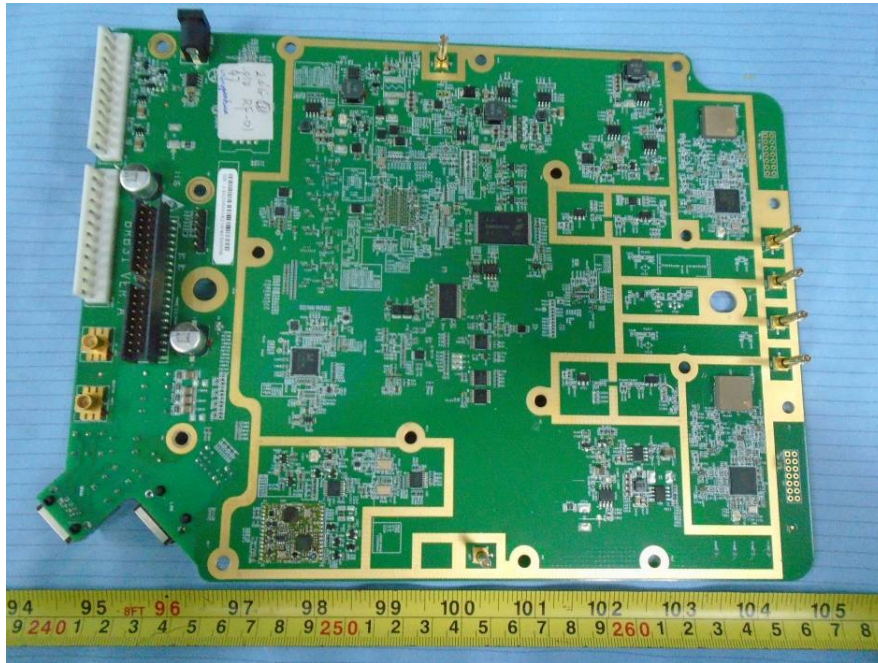
EUT – Main Board Shilding off Top View
