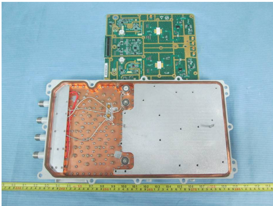
EUT –Amplifier Cover off View 2
