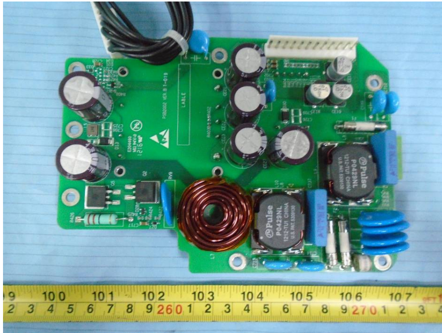
EUT –Power Main Board Top View
