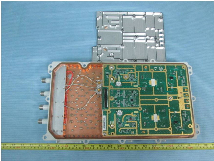
EUT –Amplifier Cover off View 1
