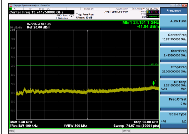
,Plot 4,2483.5MHz~25000MHz-802.11ax(H T40),2437MHz,Ant1
