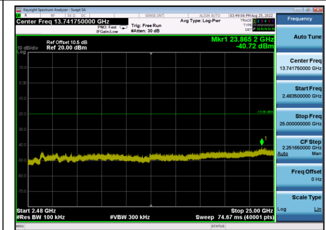
,Plot 4,2483.5MHz~25000MHz-802.11ax(H T40),2452MHz,Ant1
