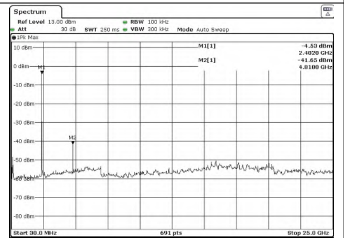
Test Mode: EDR---Low
