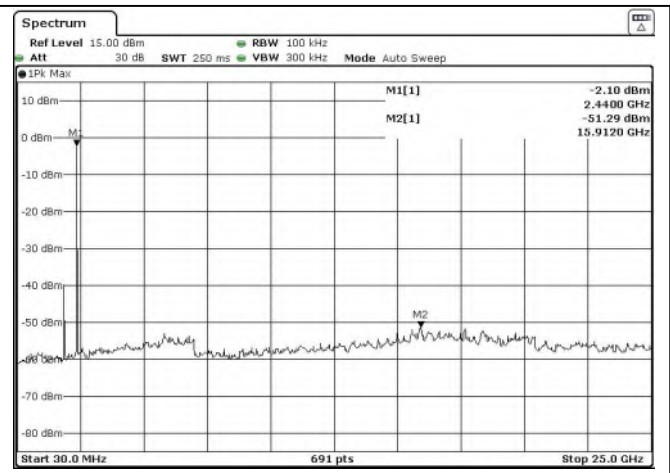
Test Mode: BDR---Mid
