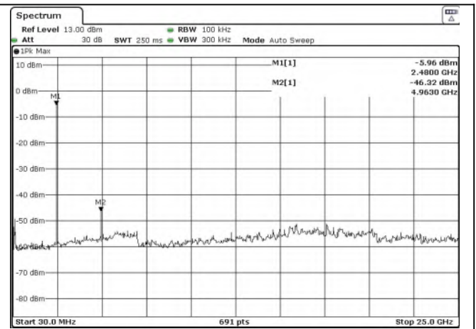
Test Mode: EDR--High
