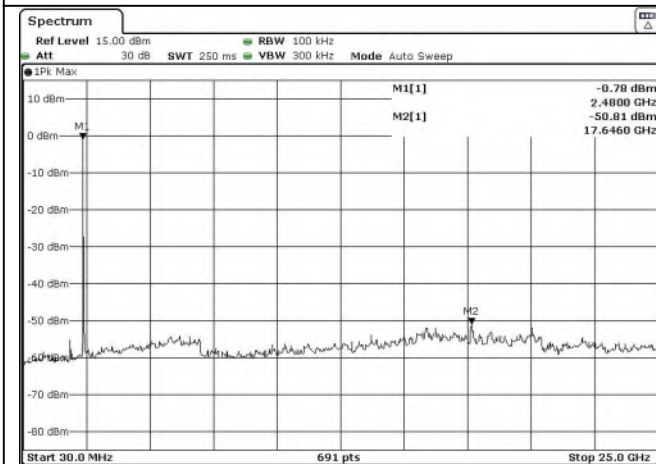
Test Mode: BDR---High
