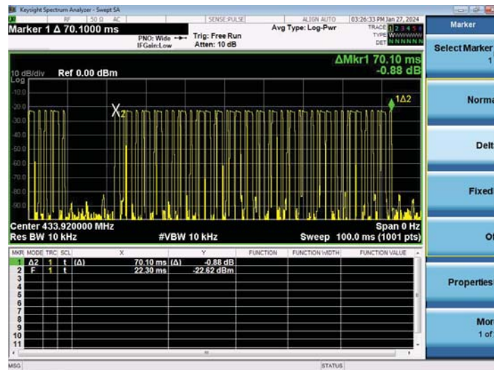
(Transmit cycle 70.10ms)
