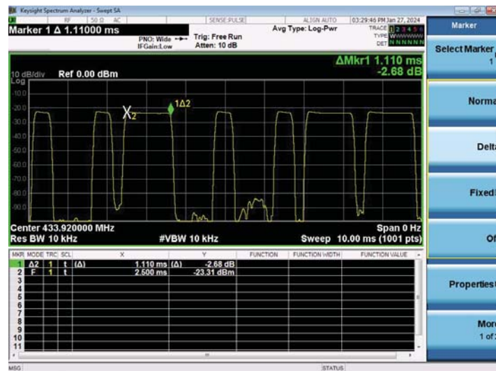
(Time per burst: 1.11ms*20pcs=22.2ms)
