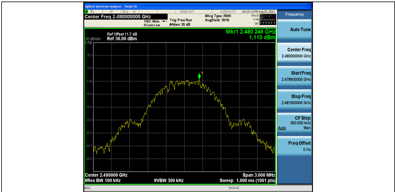
BLE_1M-Ant1-2480-0~Reference-PASS
